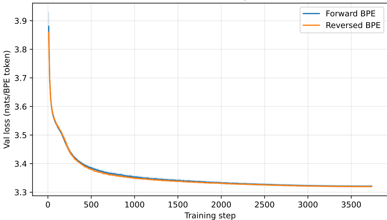
BPE Forward vs Reversed Training Dynamics (token-level reversal, same compression, 5 seeds)
