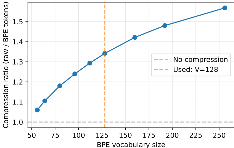
Compression vs Vocabulary Size
