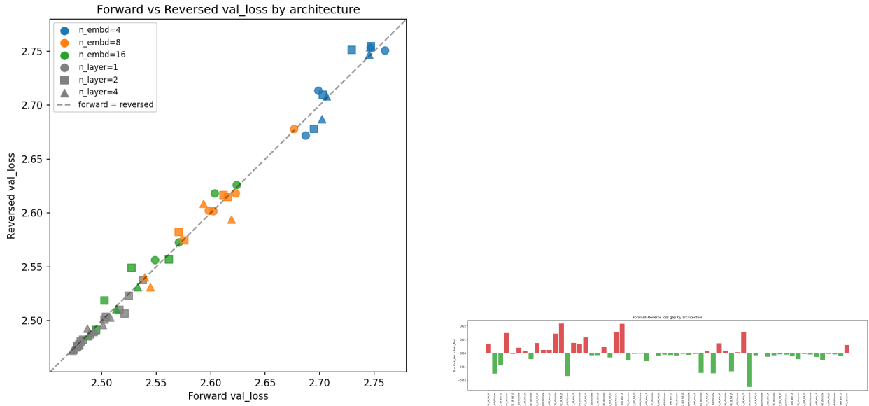
(a) Forward vs. reversed validation loss for all 60 matched configurations, coloured by n_{\text{embd}} . Points on the diagonal indicate identical performance; points above the diagonal indicate reversed sequences are harder. The data cluster tightly around the diagonal.
