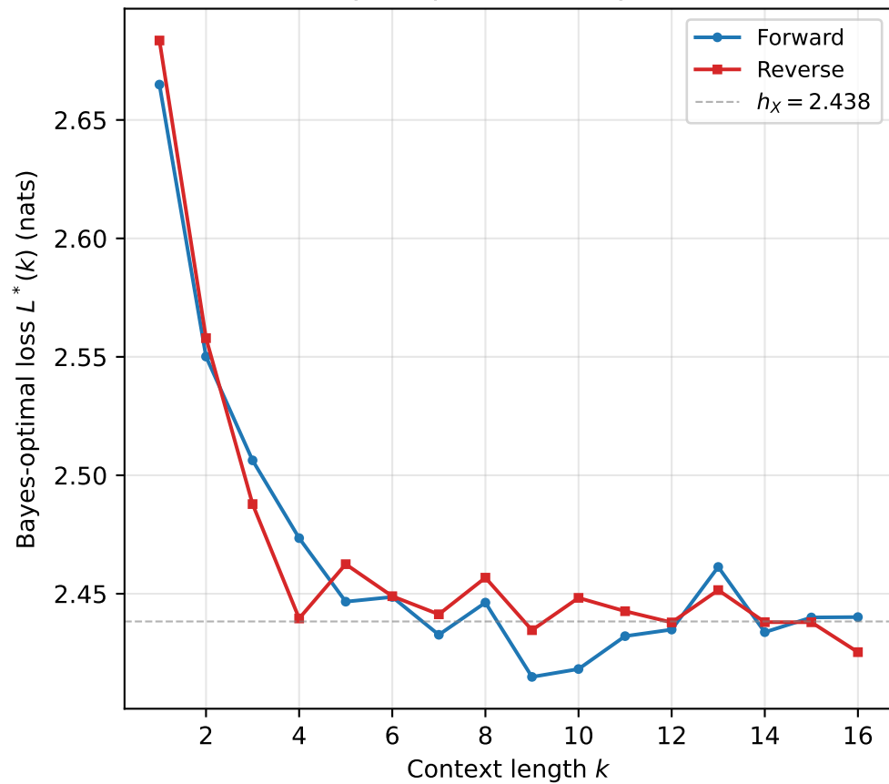
(b) Bayes-optimal loss by context
