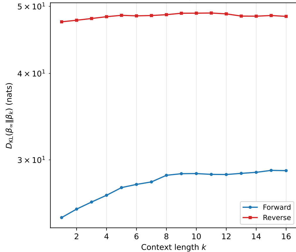
(a) Belief convergence rate
