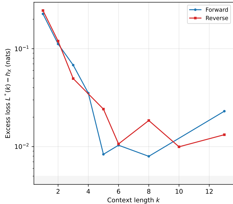
(c) Convergence to entropy rate
