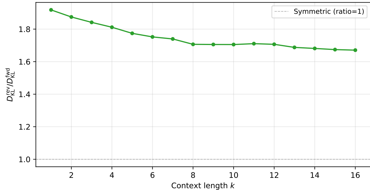
Belief convergence asymmetry ratio
