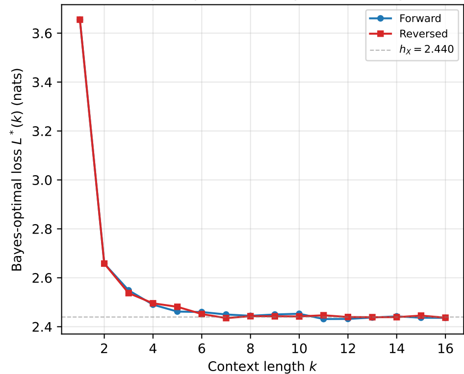
(a) Bayes-optimal loss by context length
