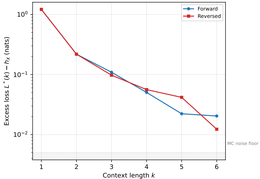
(b) Convergence to entropy rate
