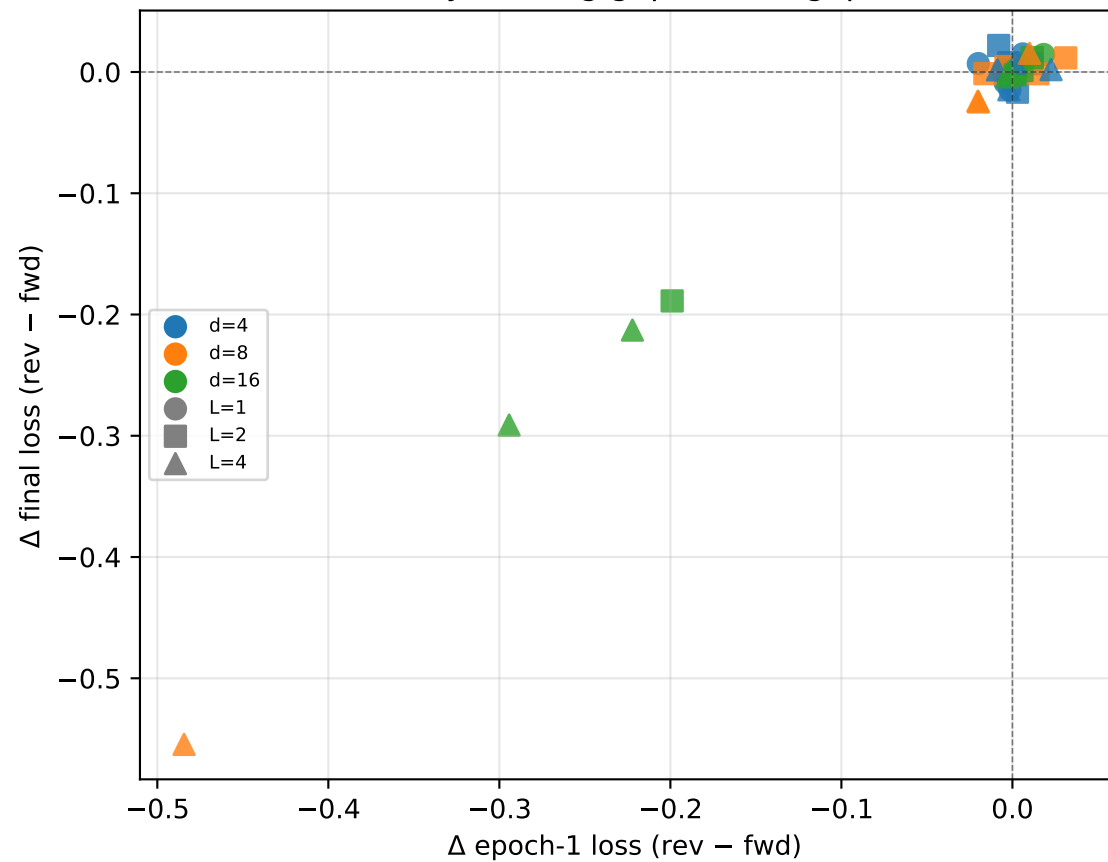
Early-training gap vs final gap
