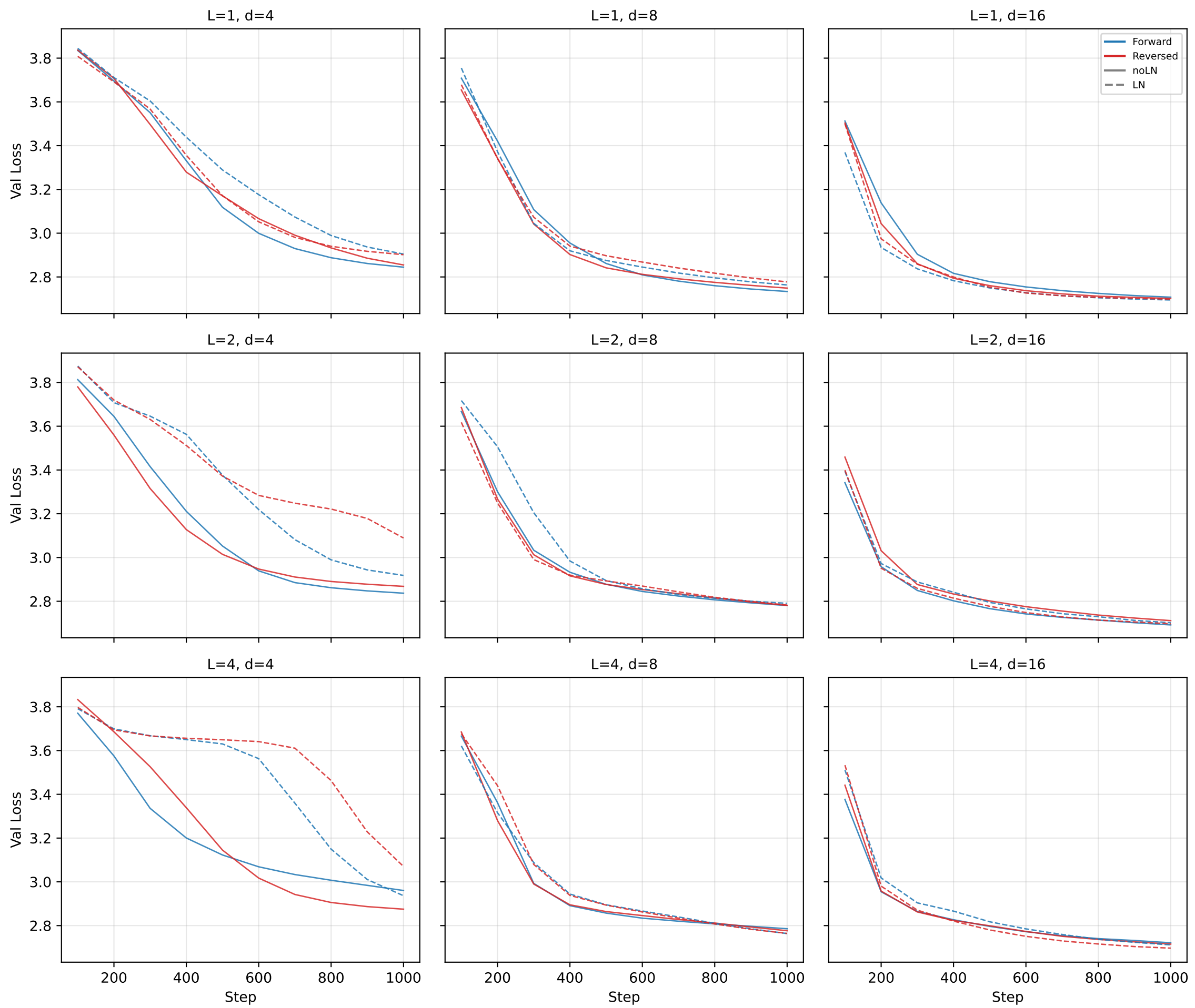
Early Training Dynamics, first 1000 steps (attn_only)
