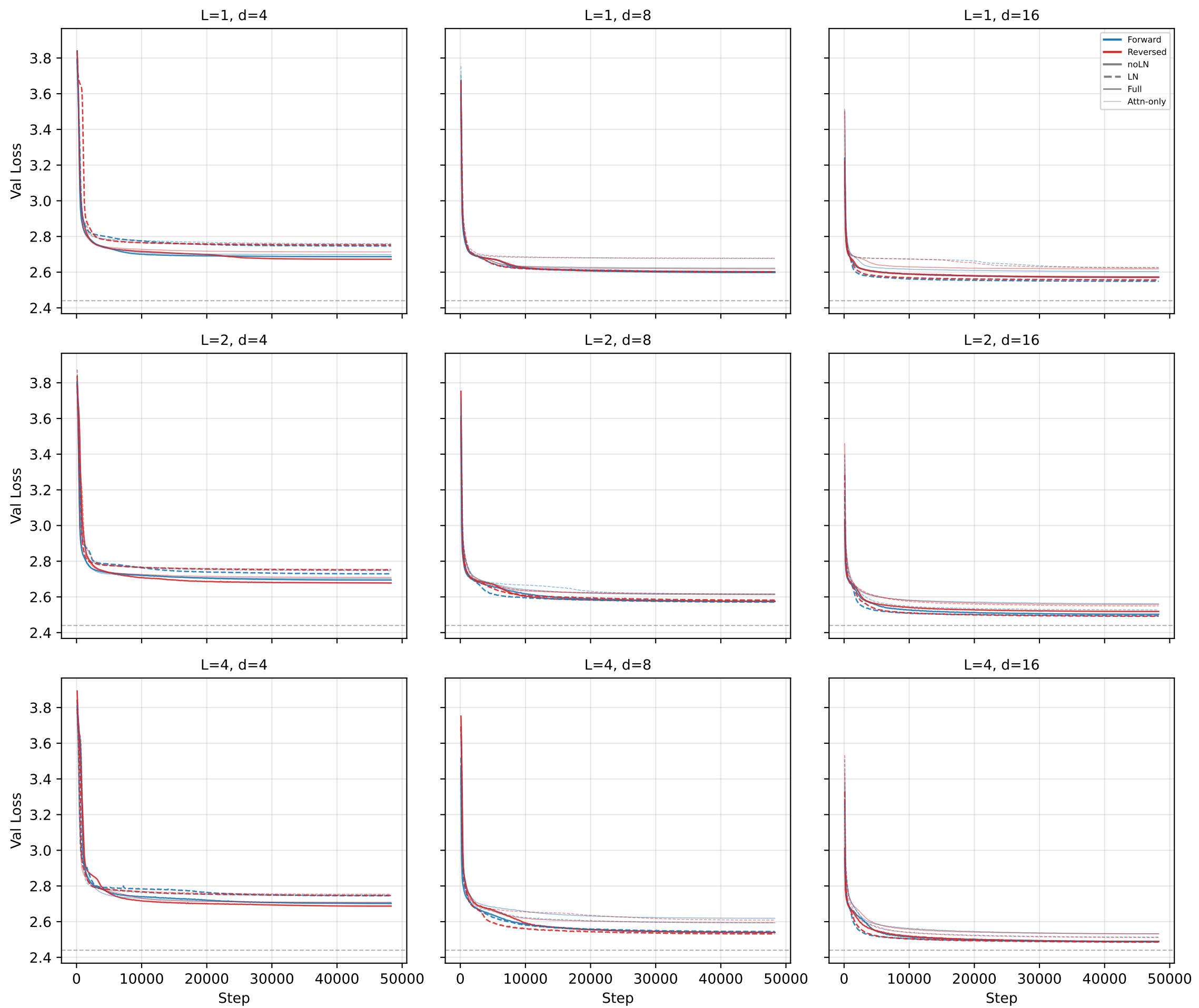
Training Dynamics: All Configs (best run per config)
