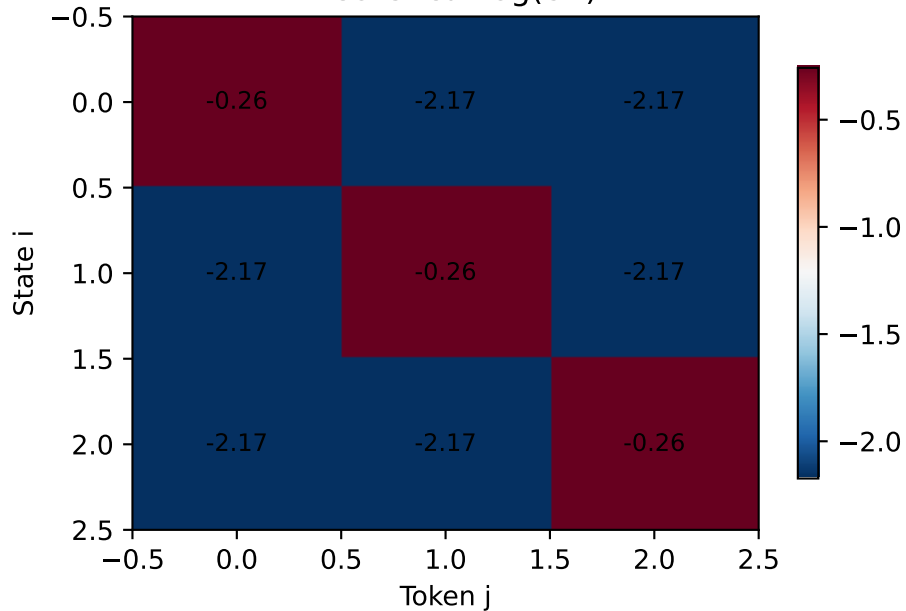
Theoretical \log(O^T)
