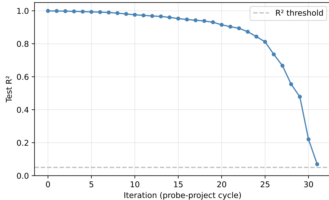
Post-LN iterative probing: R^2 after successive projections
