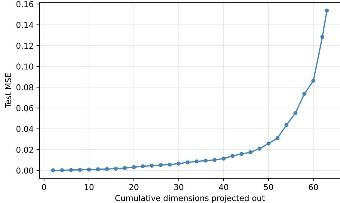
Post-LN probe MSE vs. dimensions removed
