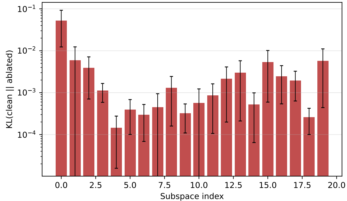
Per-subspace W_U ablation
