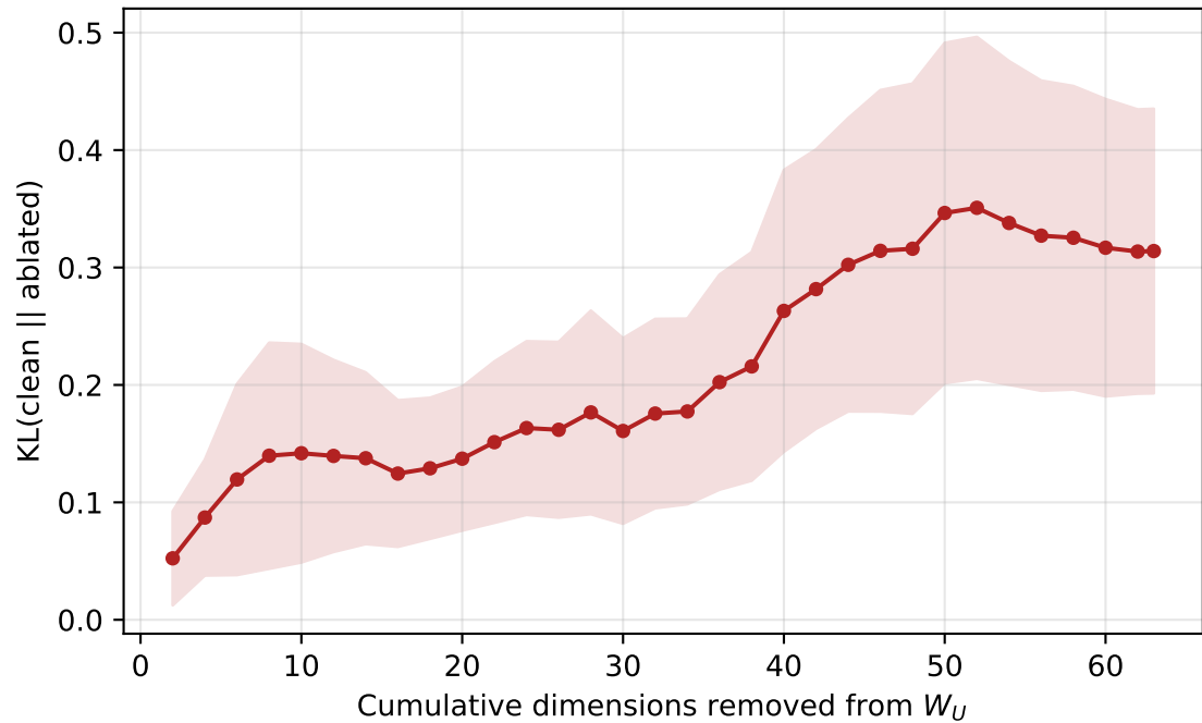
Cumulative W_U ablation
