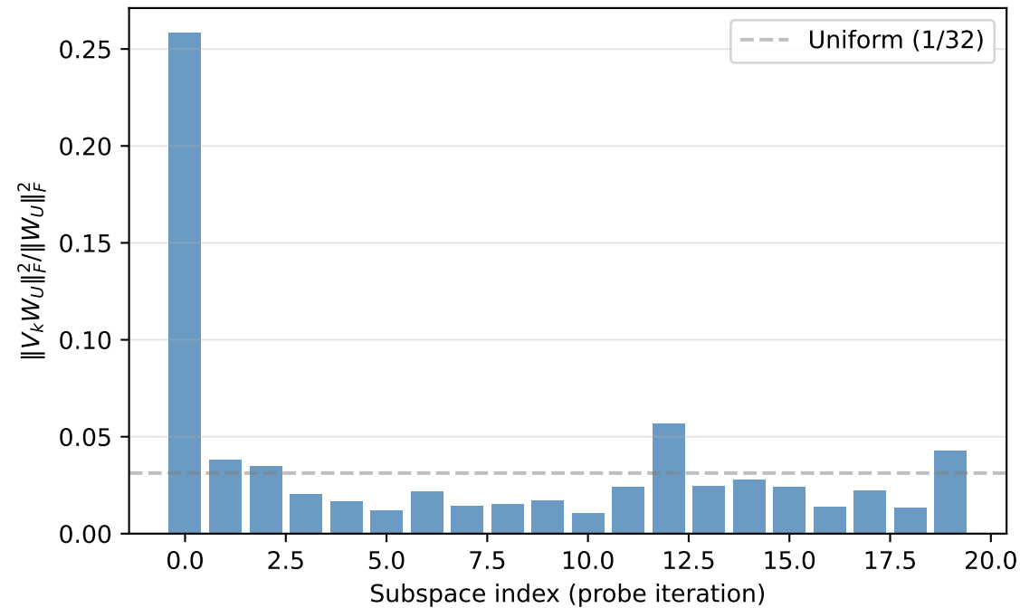
W_U overlap with each probe subspace
