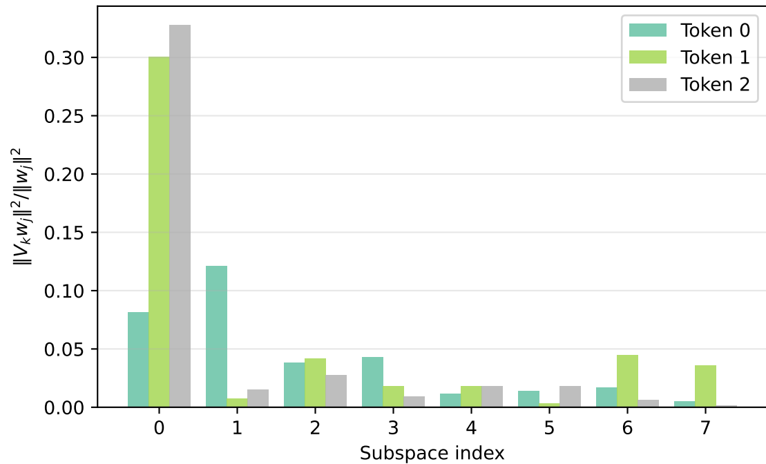
Per-token overlap breakdown
