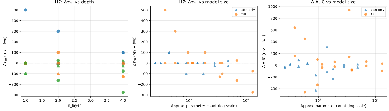
Figure B.13: Architecture dependence of training dynamics gaps. Left: \Delta\tau_{50} vs. number of layers. Centre: \Delta\tau_{50} vs. parameter count. Right: \Delta\text{AUC} vs. parameter count. Colours indicate n_{\text{embd}} (blue: 4, orange: 8, green: 16); triangles are attention-only, circles are full models.
