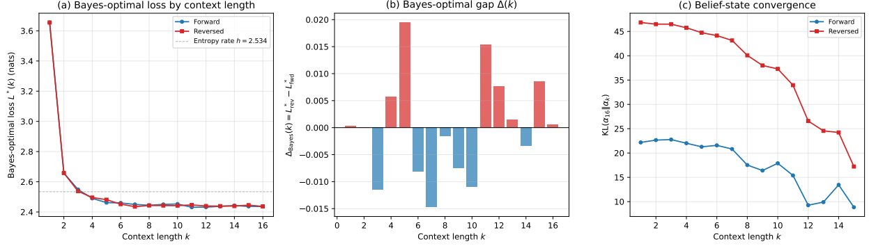
Figure B.1: Bayes-optimal analysis of forward vs. reversed CylinderGraph HMM (50,000 Monte Carlo samples). (a) Bayes-optimal loss L^*(k) converges to the entropy rate h \approx 2.534 nats for both directions by k \approx 5 . (b) The gap \Delta_{\text{Bayes}}(k) fluctuates around zero at larger k due to Monte Carlo noise; at k = 16 it is +0.0006 nats. (c) Belief-state KL divergence from the converged belief ( k = 16 ) is consistently \sim 2\times larger for the reverse process, confirming H2.
