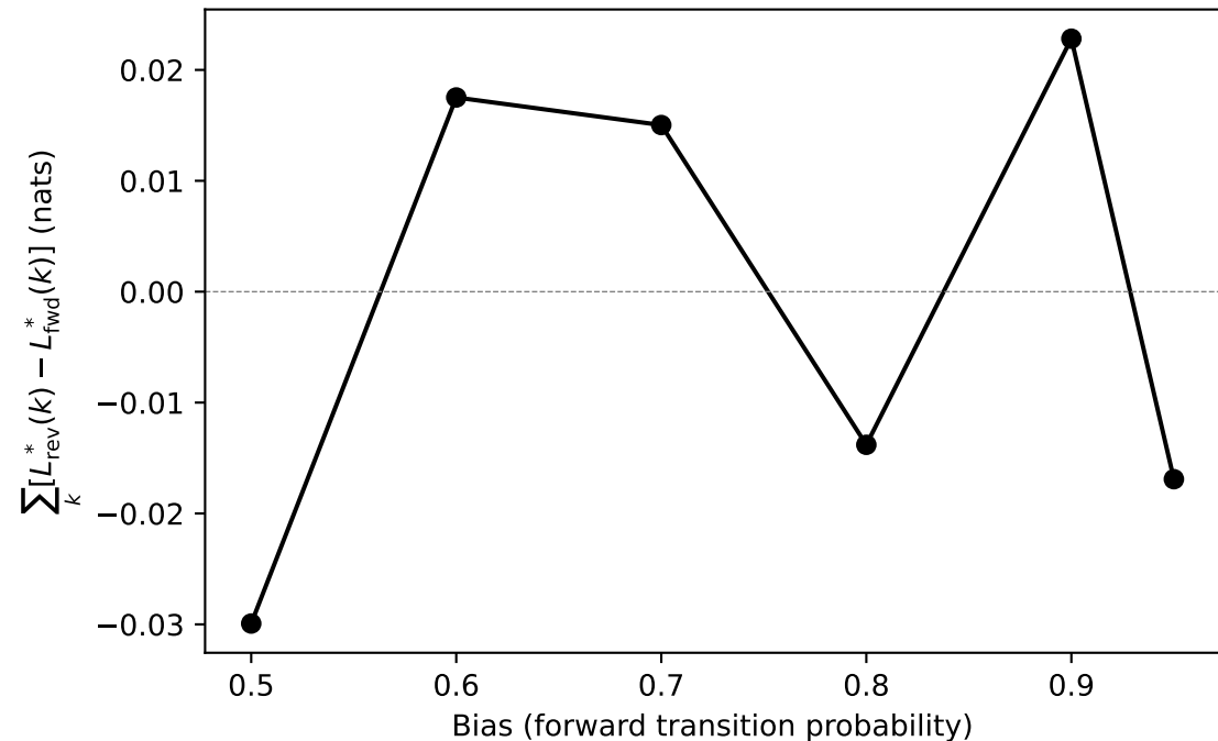
DirectedCycleHMM (N=5, noise=0.3): Integrated asymmetry gap
