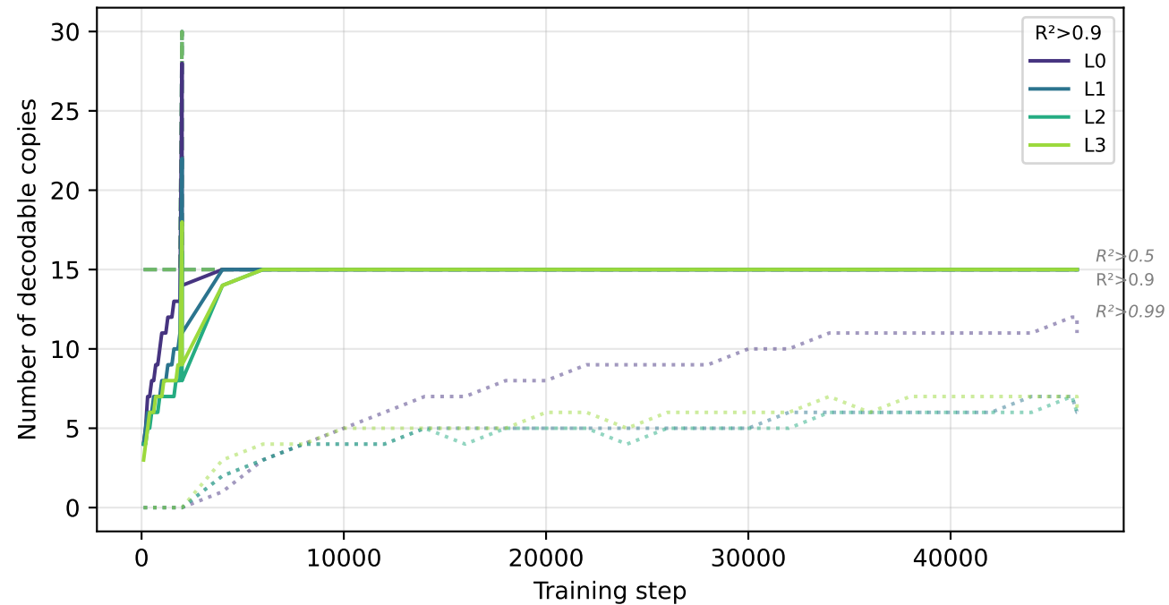
Emergence of decodable copies during training
