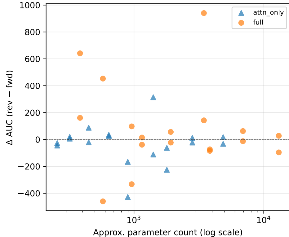
\Delta \text{AUC} vs model size
