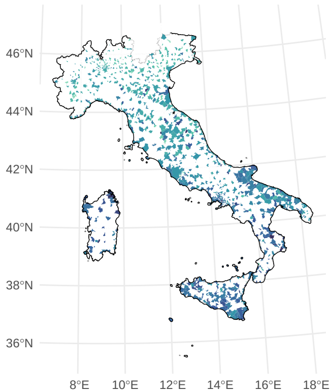
Mathematics Score
