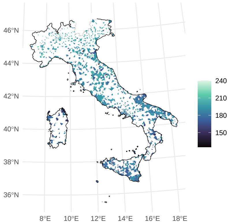
Italian Score
