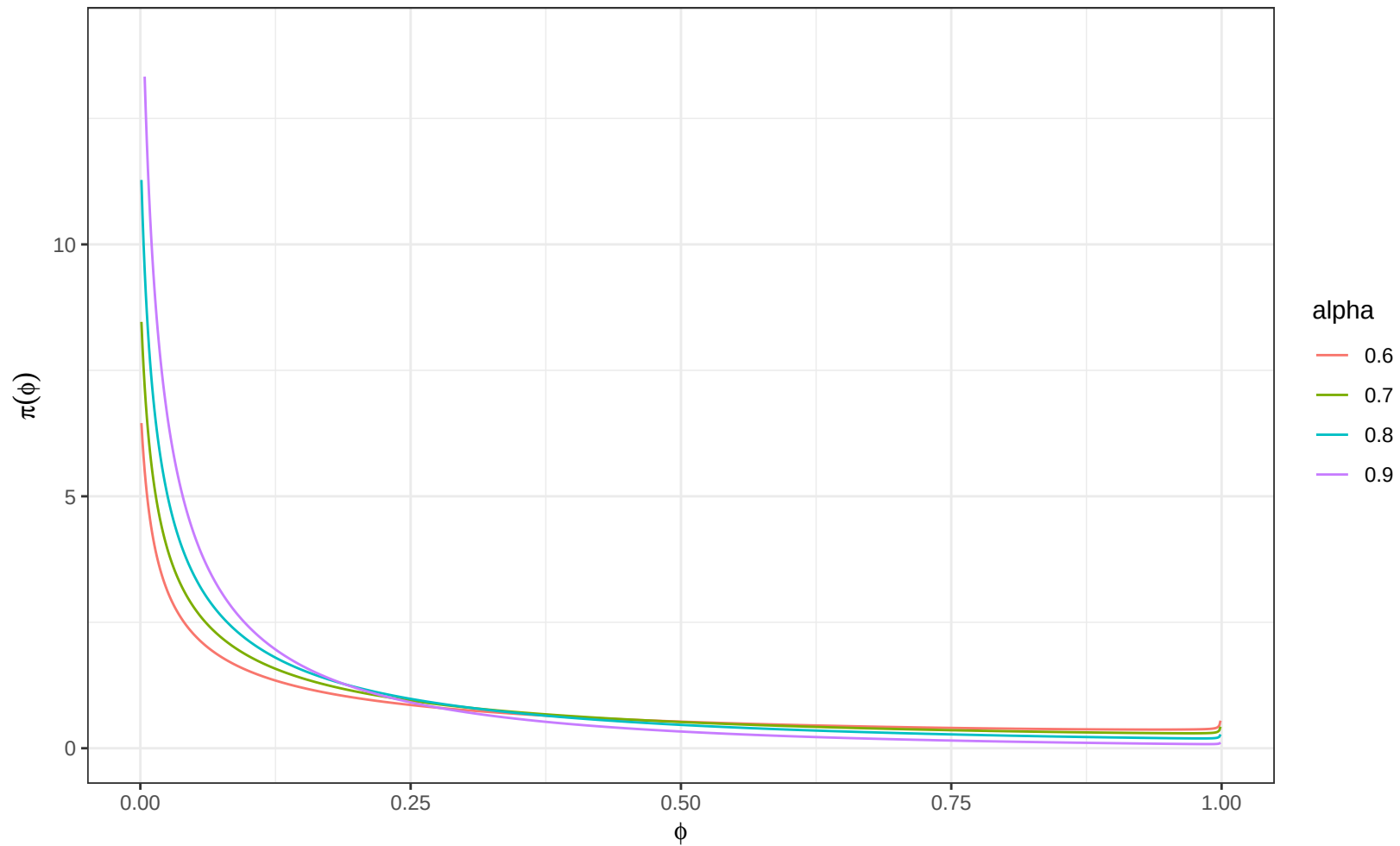
PC-prior for PCAR spatial autocorrelation parameter with U=0.5
