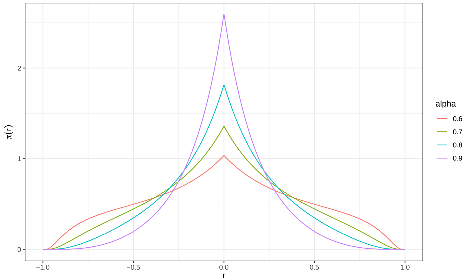
PC-prior for AR(1) autocorrelation parameter with U=0.4
