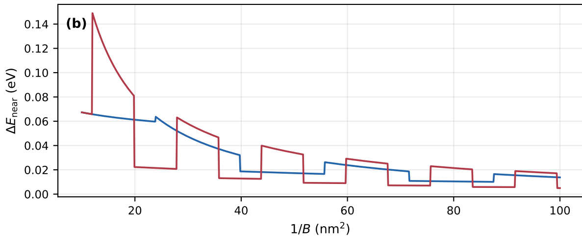
LL spacing closest to \mu_S
