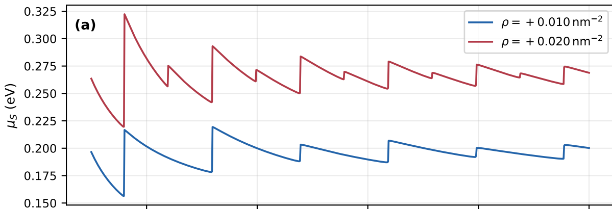
LL spacing closest to \mu_S
