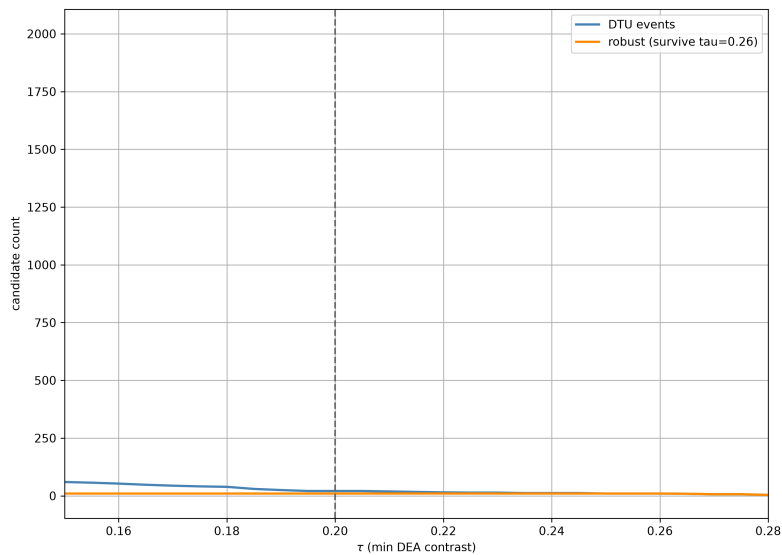
Figure 4.5: Zoomed tau sensitivity sweep for the human dataset over 0.15 \leq \tau \leq 0.28 , chosen so the descending slope and the stable plateau are both visible in one panel. Total DTU events descend from 60 at \tau = 0.15 through 21 at \tau = 0.2 , then fall further until they meet the robust core at \tau = 0.25 ; from 0.25 to 0.26 both counts hold flat at ten—the genuine plateau. The published threshold \tau = 0.2 (dashed) sits at the foot of the slope, just below that highland.
