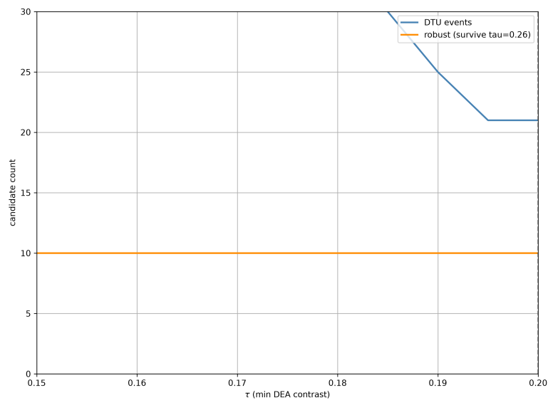
Figure 4.5: Zoomed tau sensitivity sweep for the human dataset over 0.15 \leq \tau \leq 0.2 (y-axis restricted to 0–30). Total DTU events descend from 60 to 21 with no local plateau, but the robust-core count holds flat at ten across the entire interval: even as the total candidate set shrinks, the stable core of switches does not change. The published threshold \tau = 0.2 (dashed) sits at the foot of the slope, just below the stable highland at \tau = 0.25 .
