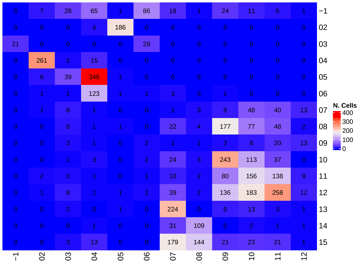
Transcript Clusters
