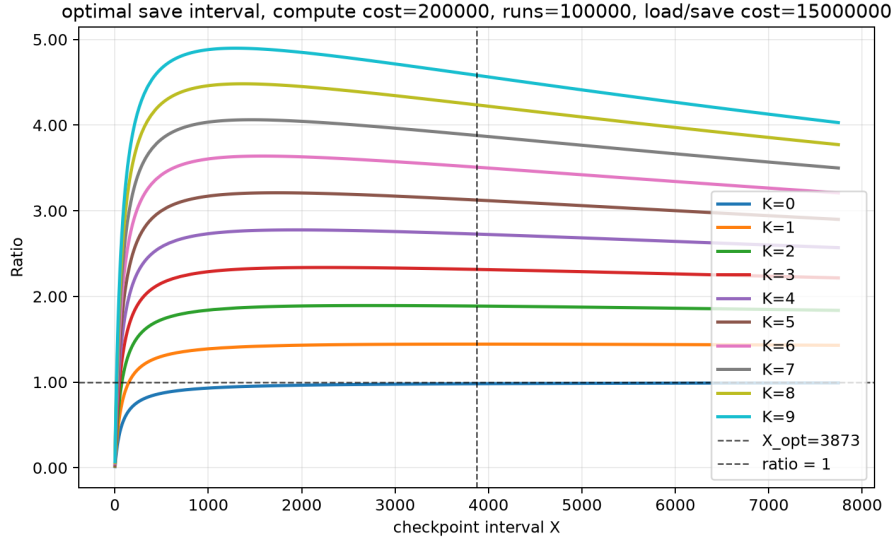
Figure 6.9: Optimal checkpoint interval for 100k runs and 1 error , over for k=[0 - 9] , 15m load/save cost and 200k compute cost
