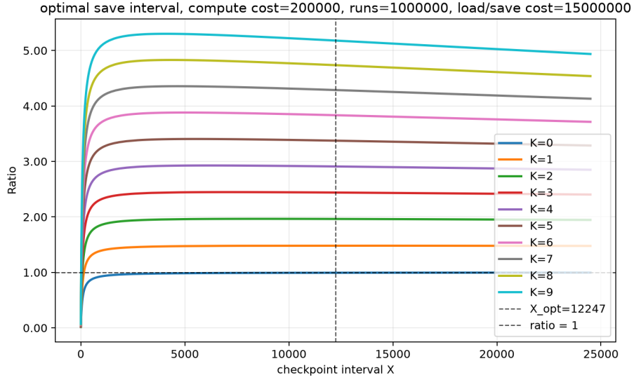
Figure 6.10: Optimal checkpoint interval for 1m runs and 1 fault , over for k=[0-9] , 15m load/save cost and 200k compute cost
