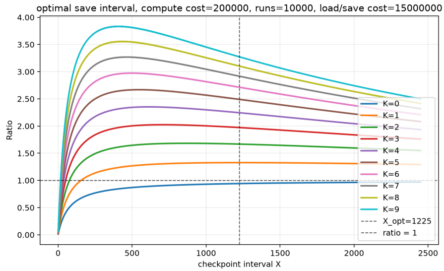
Figure 6.8: Optimal checkpoint interval for 10k runs and 1 error , over for k=[0-9] , 15m load/save cost and 200k compute cost
