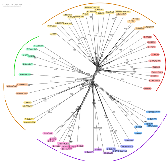
Genome-wide nucleotide network
