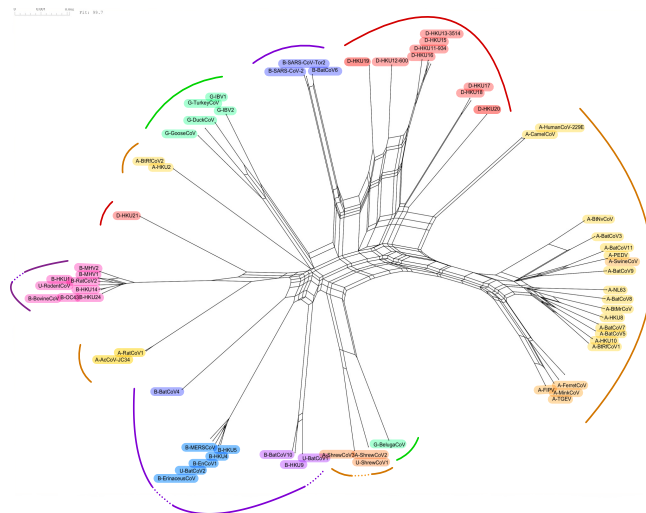
S-gene indel network
