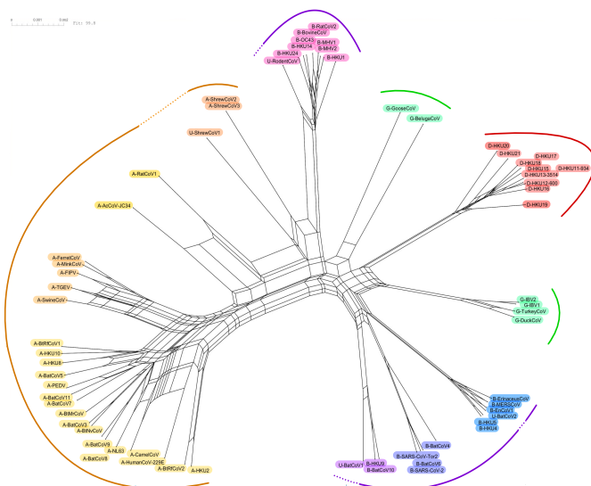
Genome-wide indel network
