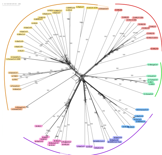
S-gene nucleotide network
