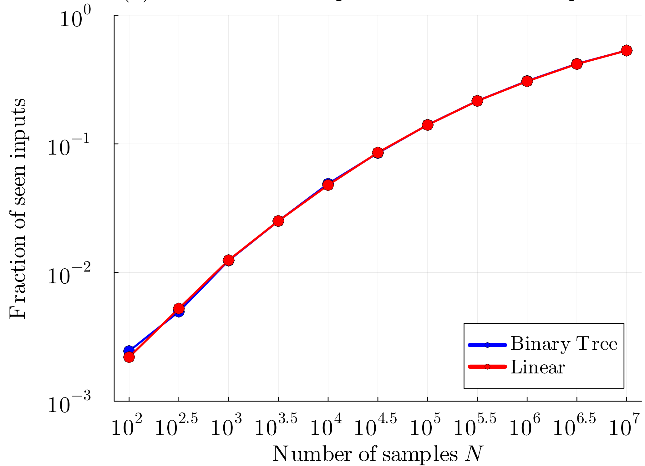
(b) Fraction of seen inputs vs. Number of samples N
