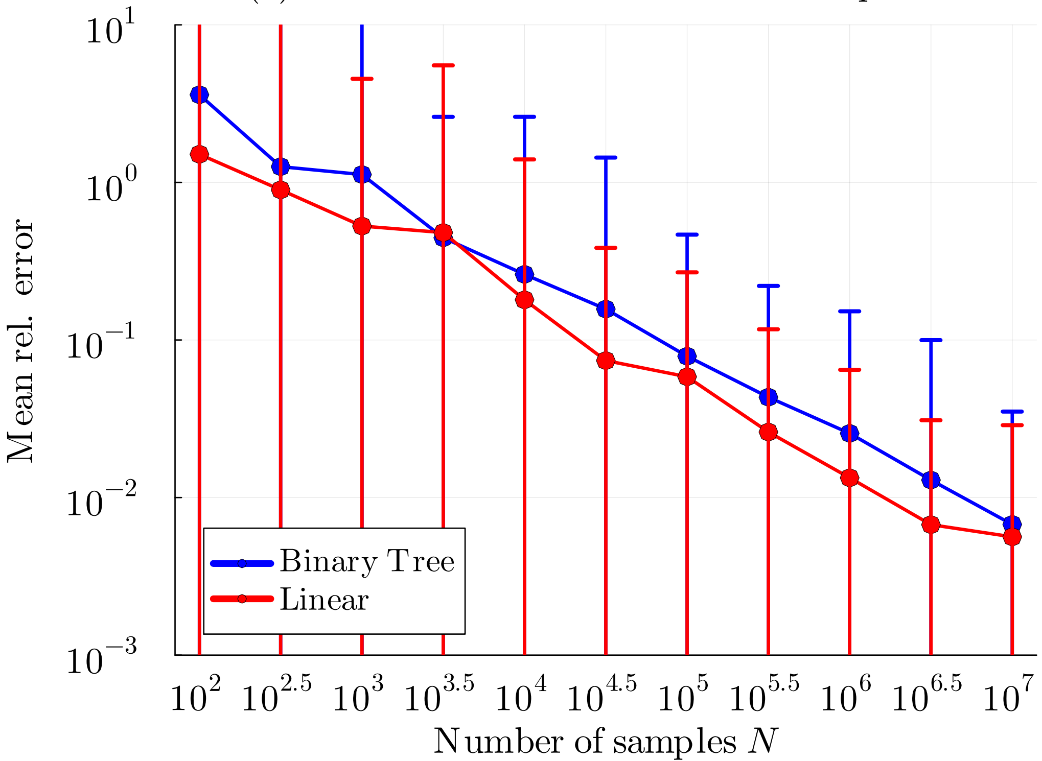
(a) Mean rel. error vs. Number of samples N
