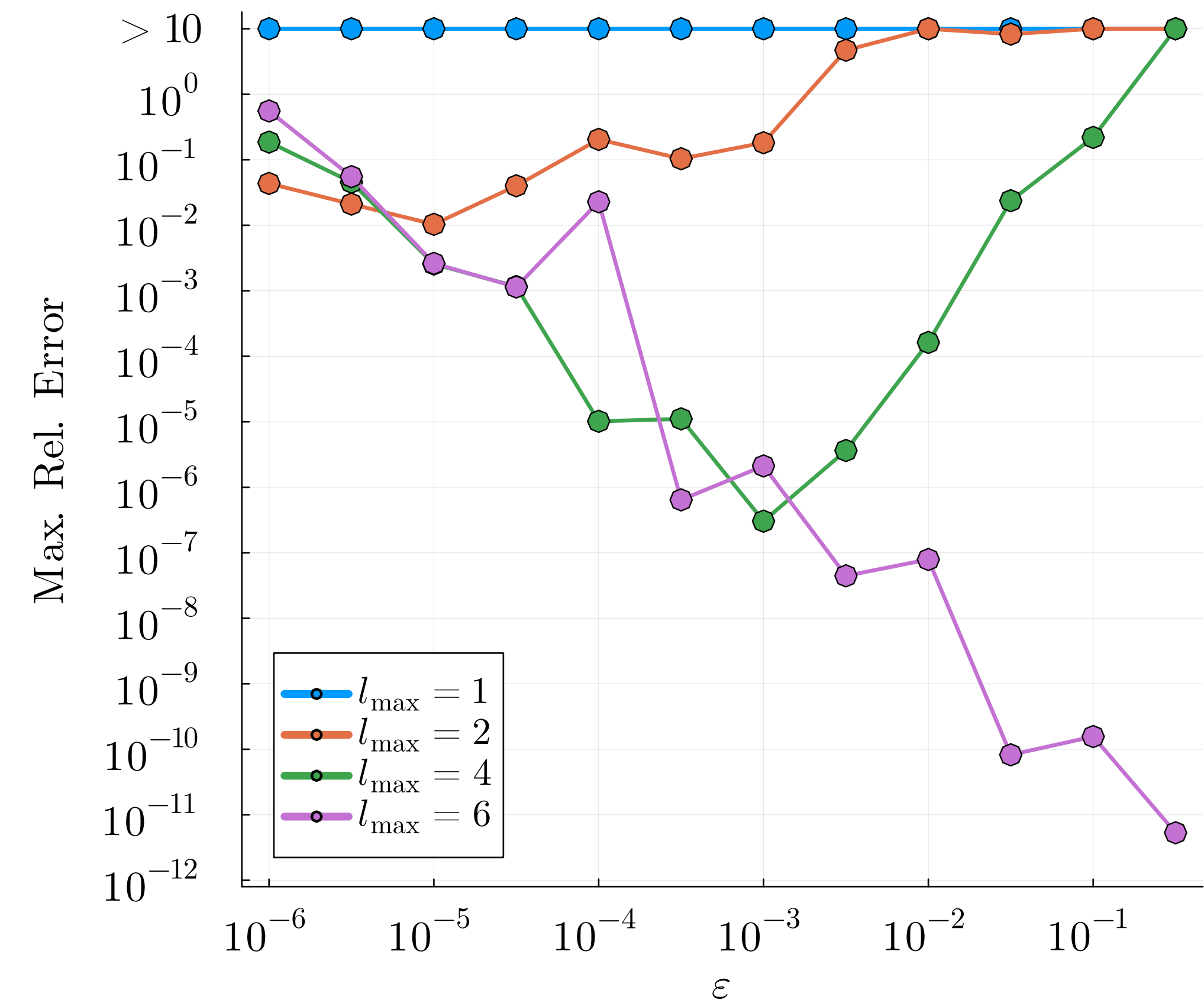
(a) Max. Rel. Error vs. \varepsilon , ( n_{\text{Cond.}} = 1 )
