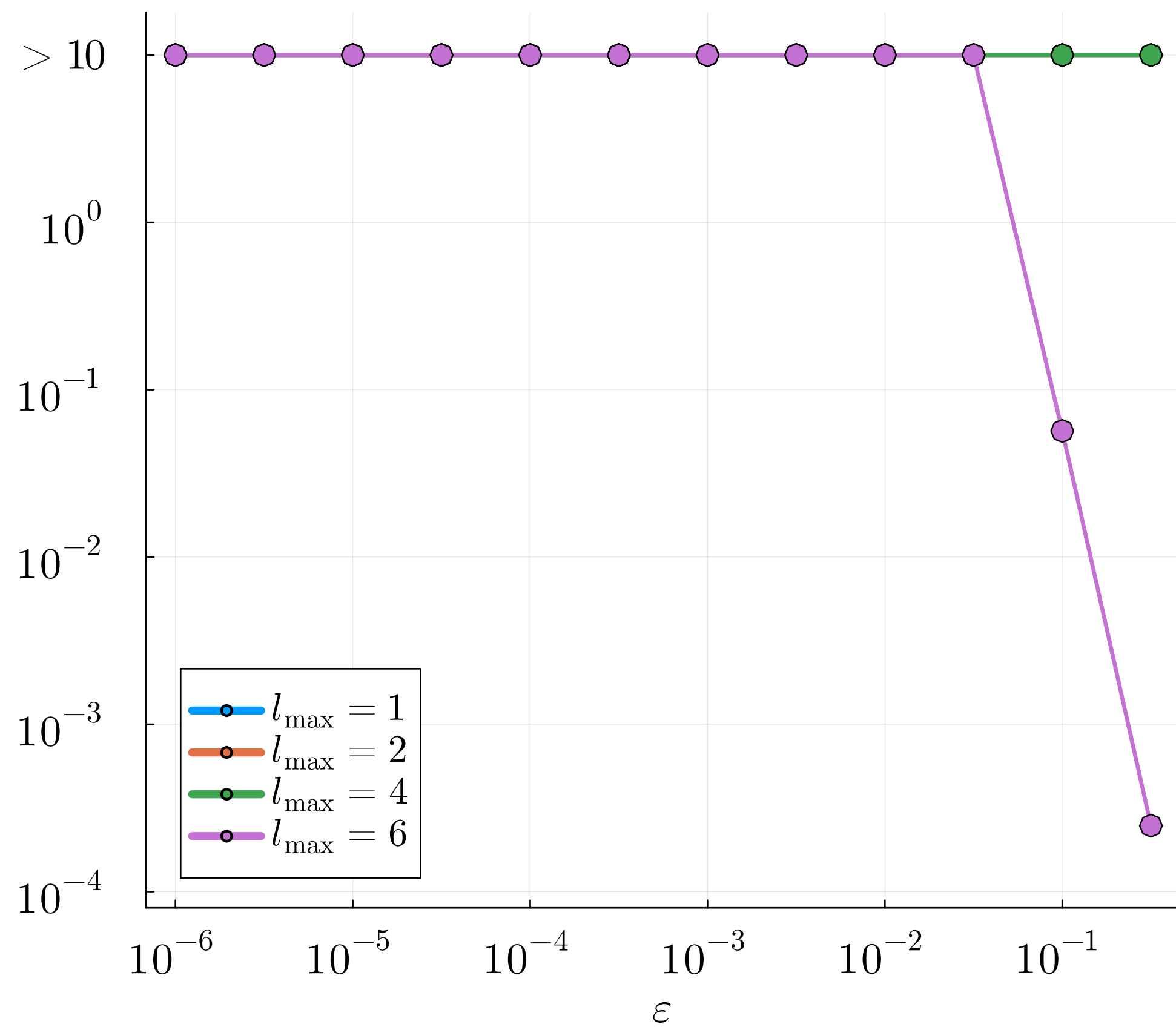
(c) Max. Rel. Error, n_{\text{Cond}} = 3
