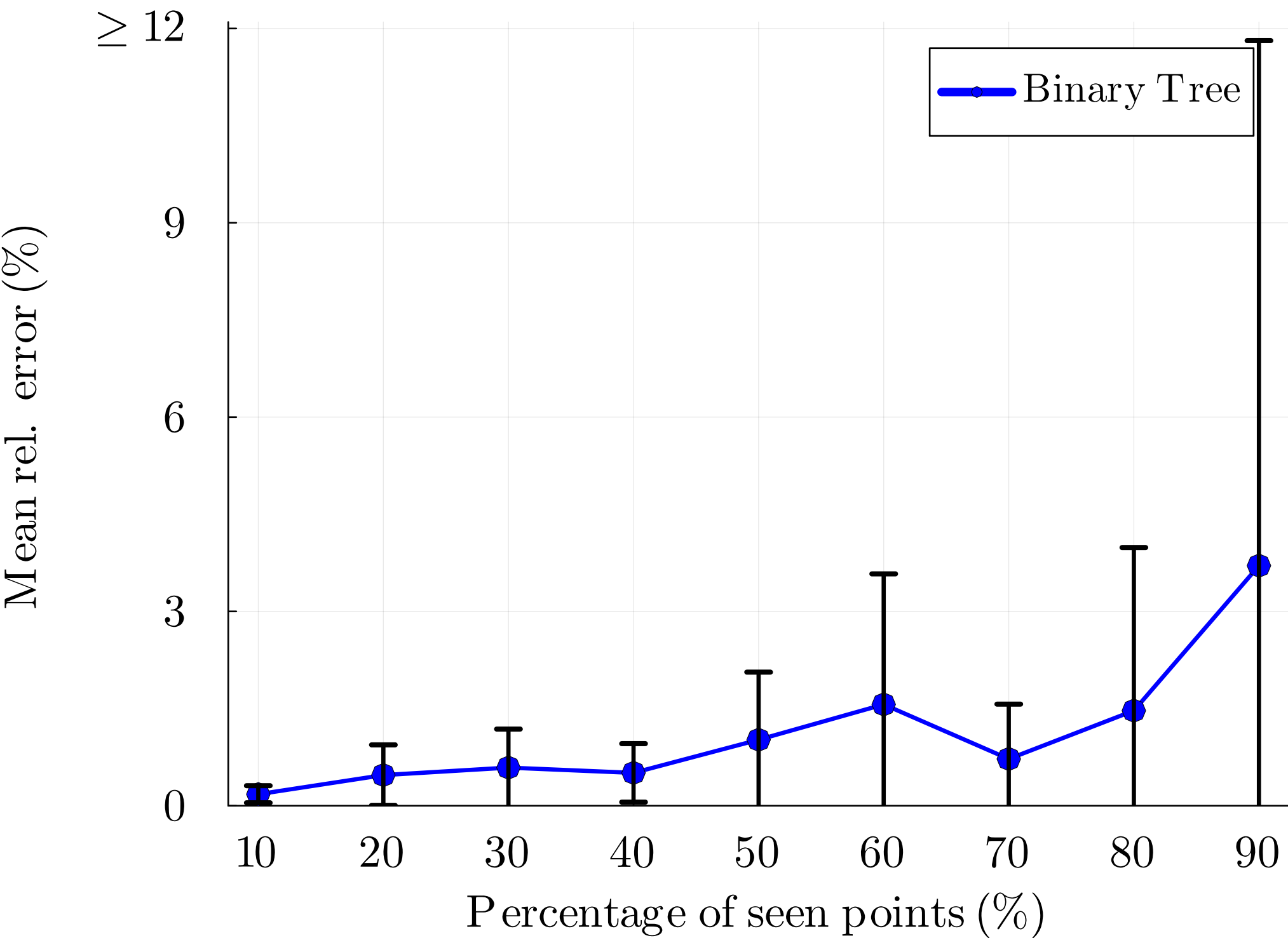
(a) Binary tree (15 vertices)
