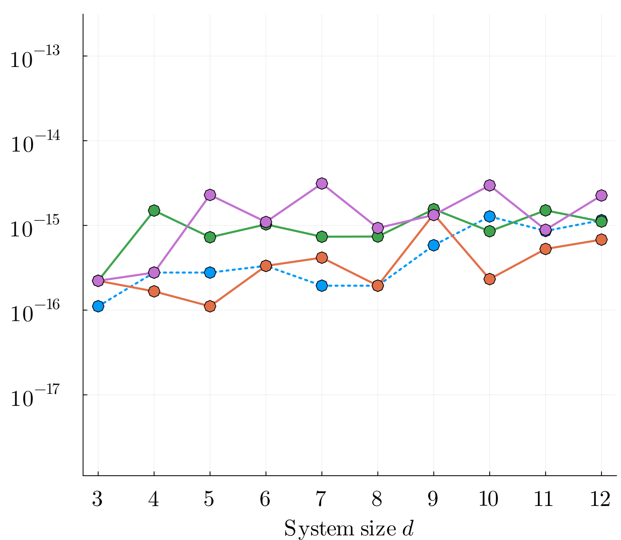
(b) Max. Abs. Error \max_x |f(x) - f_{\text{ttns}}(x)|
