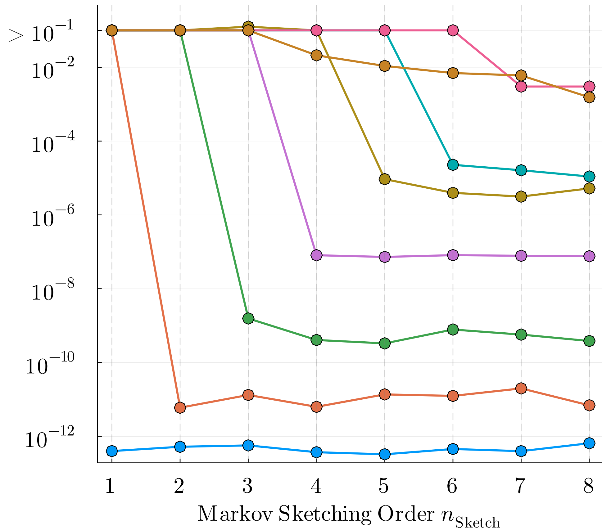
(a) Max. Rel. Error \max_x |(f(x) - f_{\text{ttns}}(x))| / f(x)
