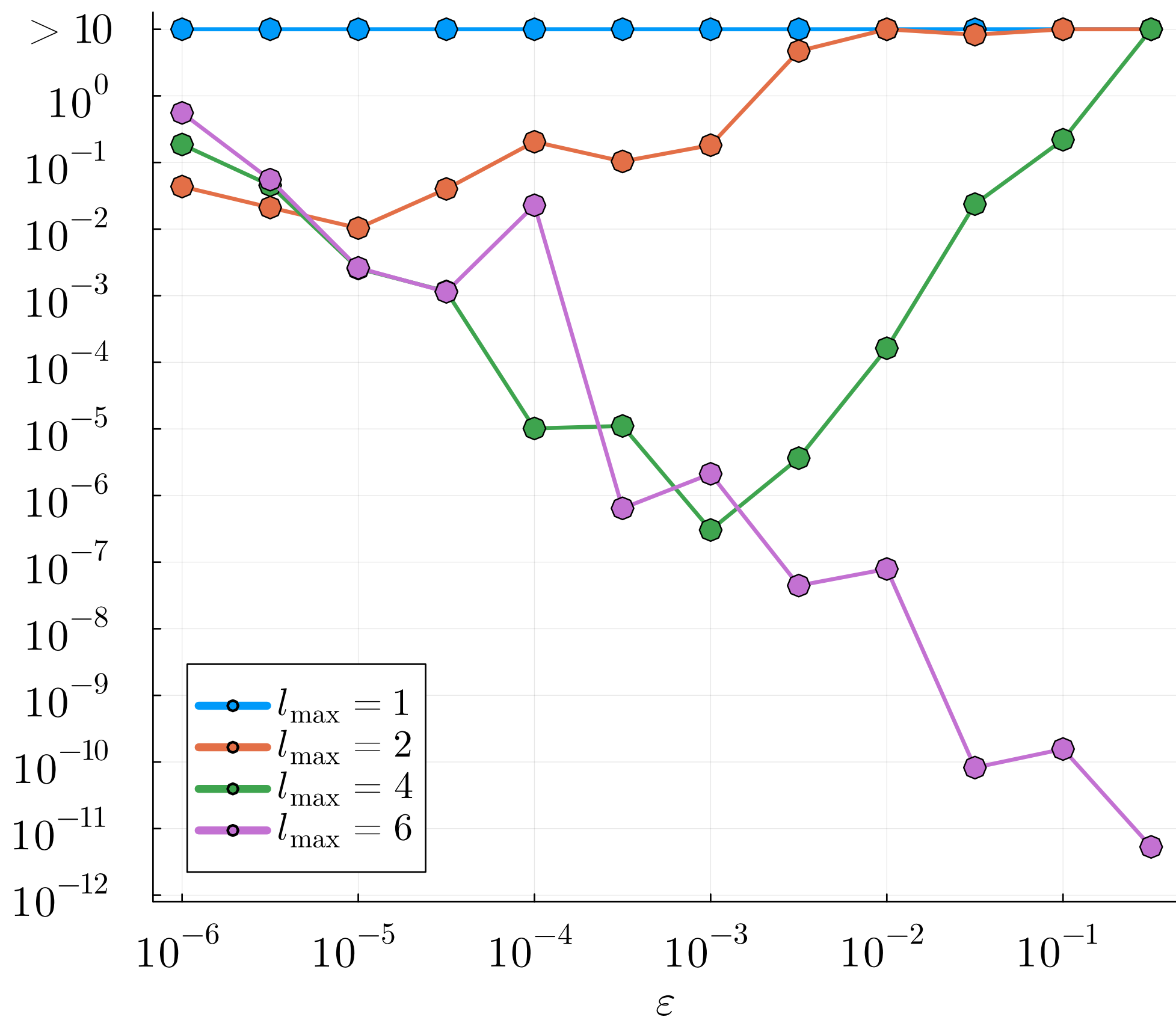
(a) Max. Rel. Error, n_{\text{Cond}} = 1
