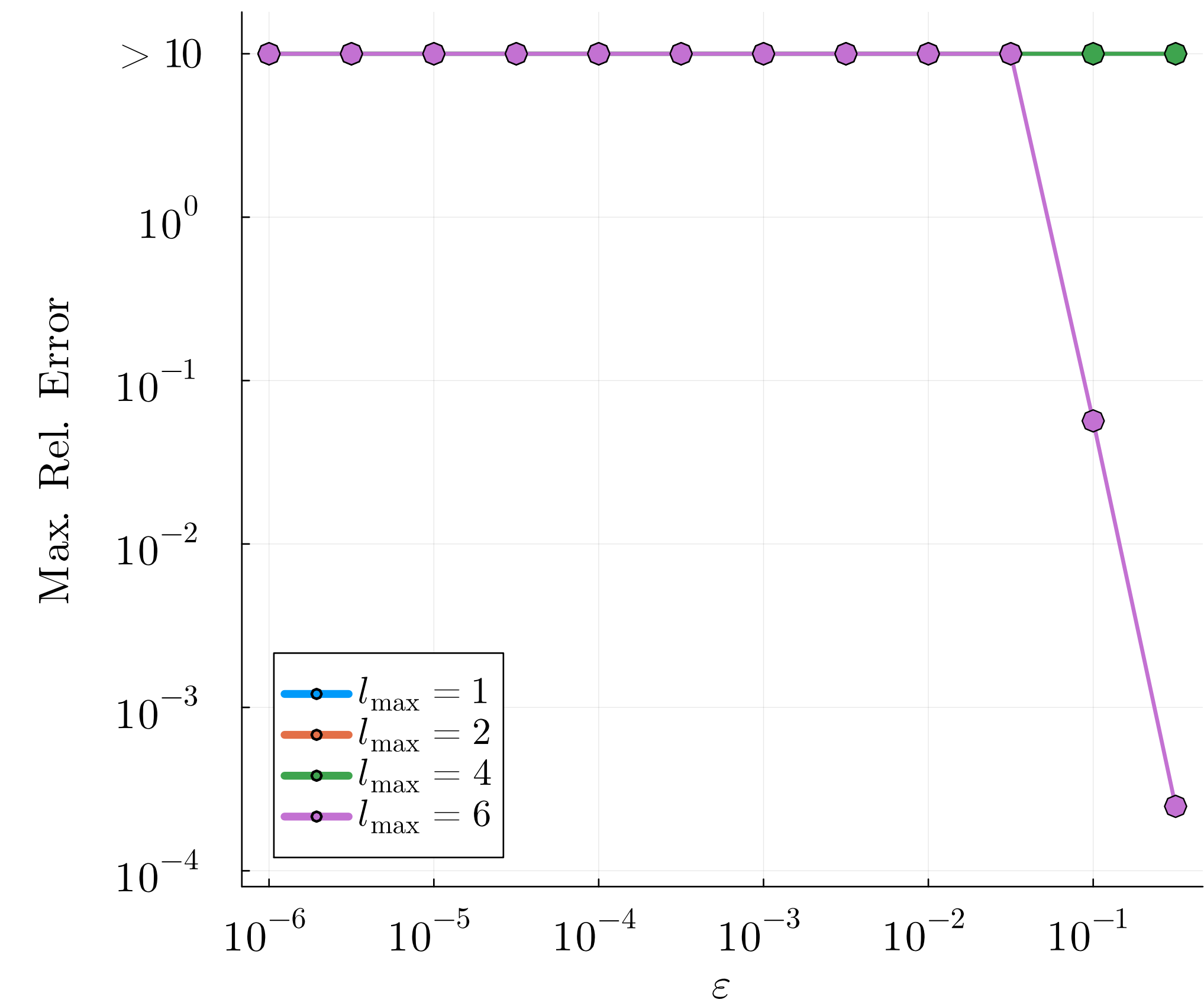
(c) Max. Rel. Error vs. \varepsilon , ( n_{\text{Cond.}} = 3 )
