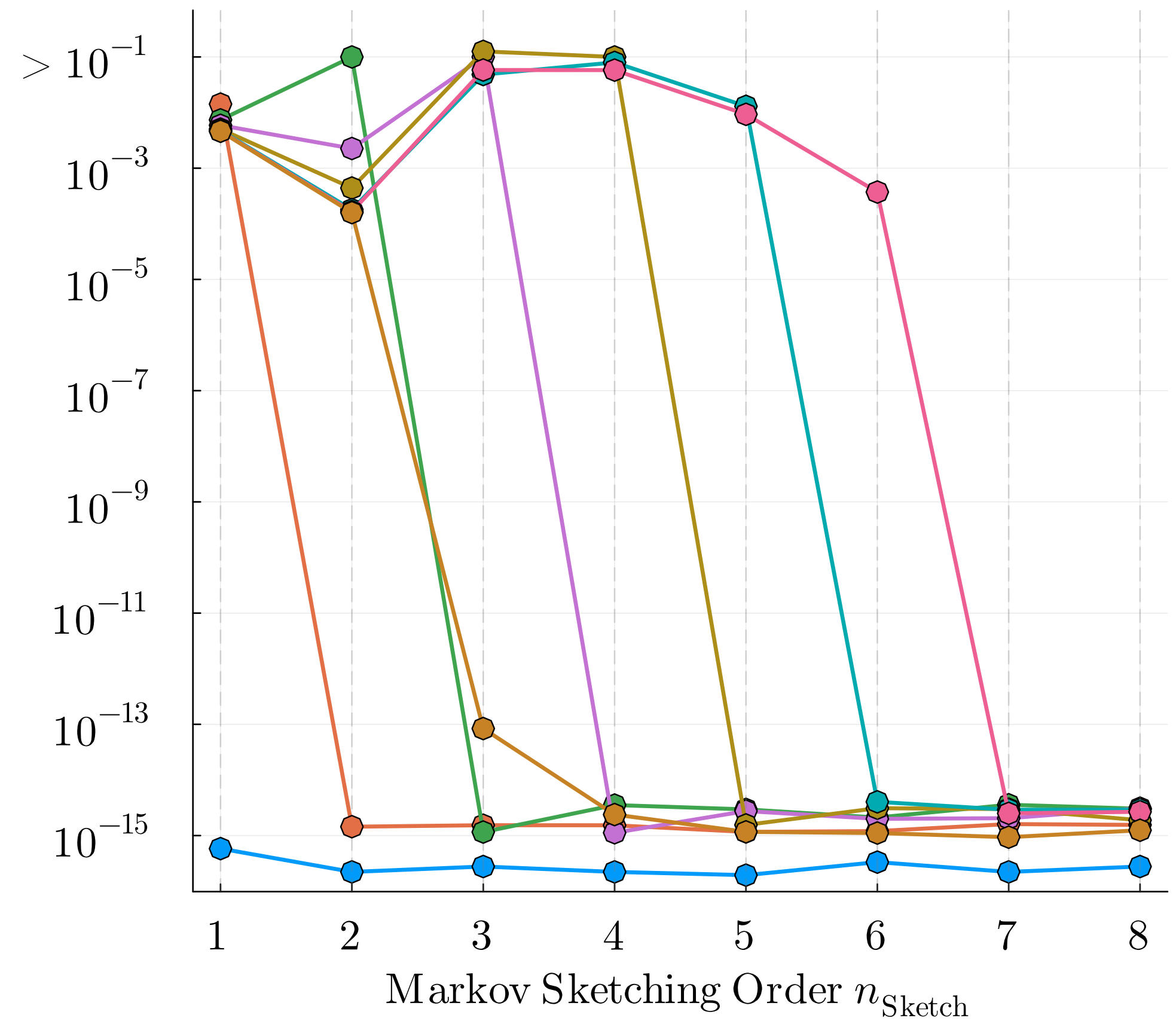
(b) Max. Abs. Error \max_x |f(x) - f_{\text{ttns}}(x)|
