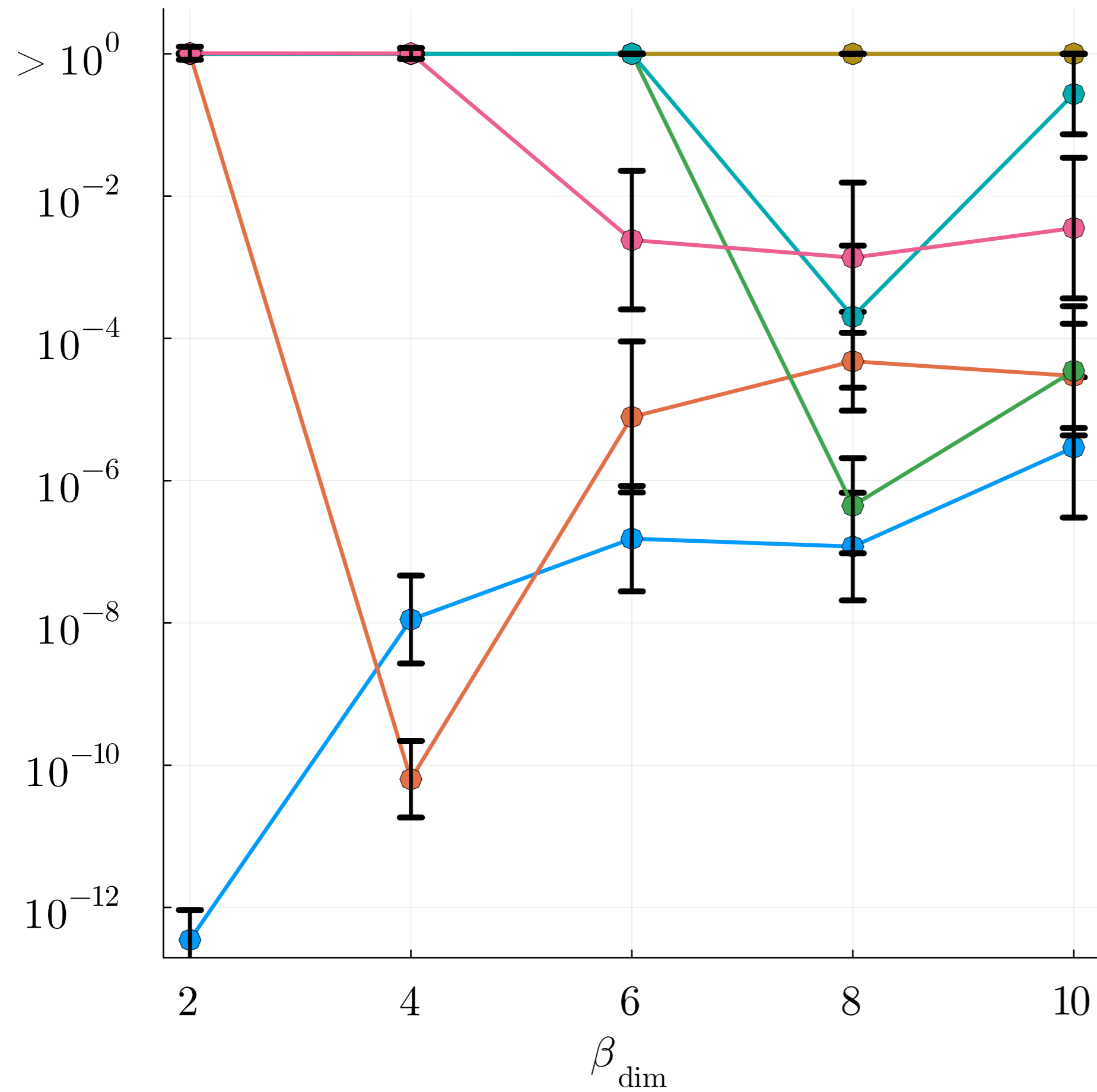
(a) Perturbative Sketching : Rel. error vs. \beta_{\text{dim}}
