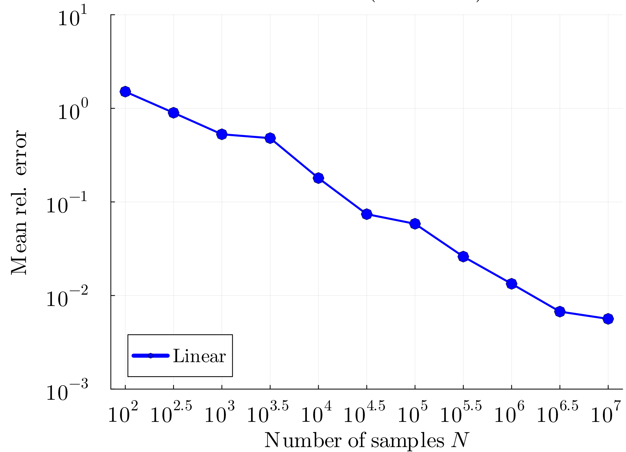
Linear chain (15 vertices)
