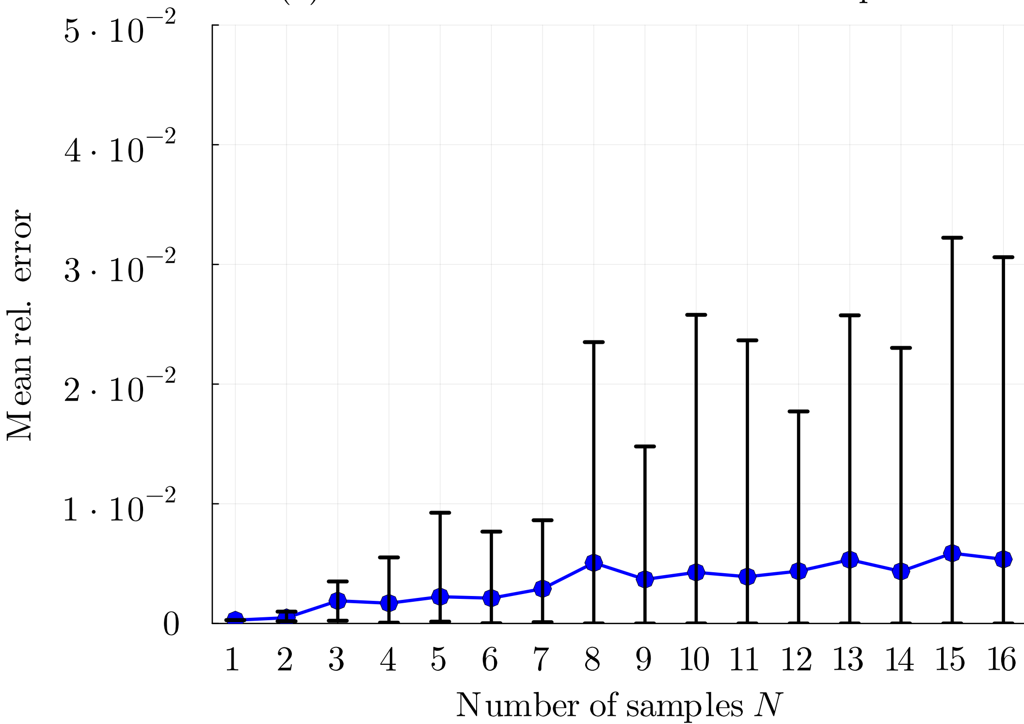
(a) Mean rel. error vs. Number of samples N
