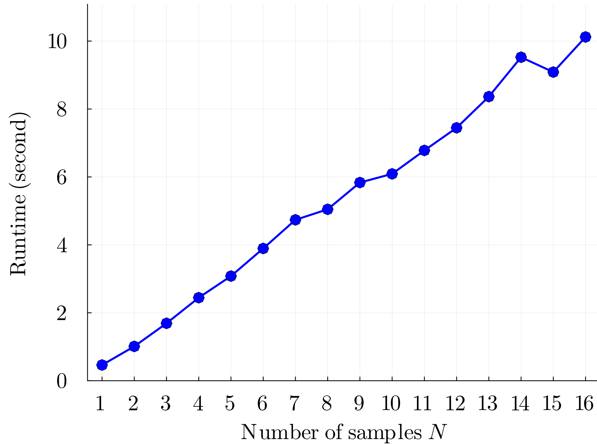
(b) Runtime vs. Number of samples N
