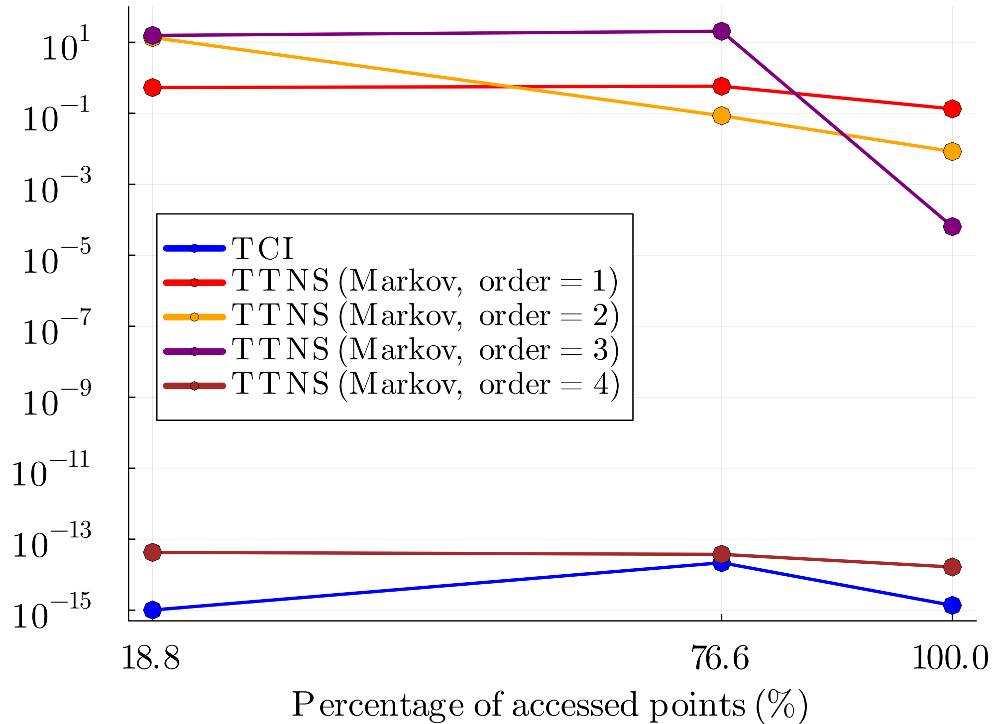
Seen points : Max. rel. error vs. frac. accessed
