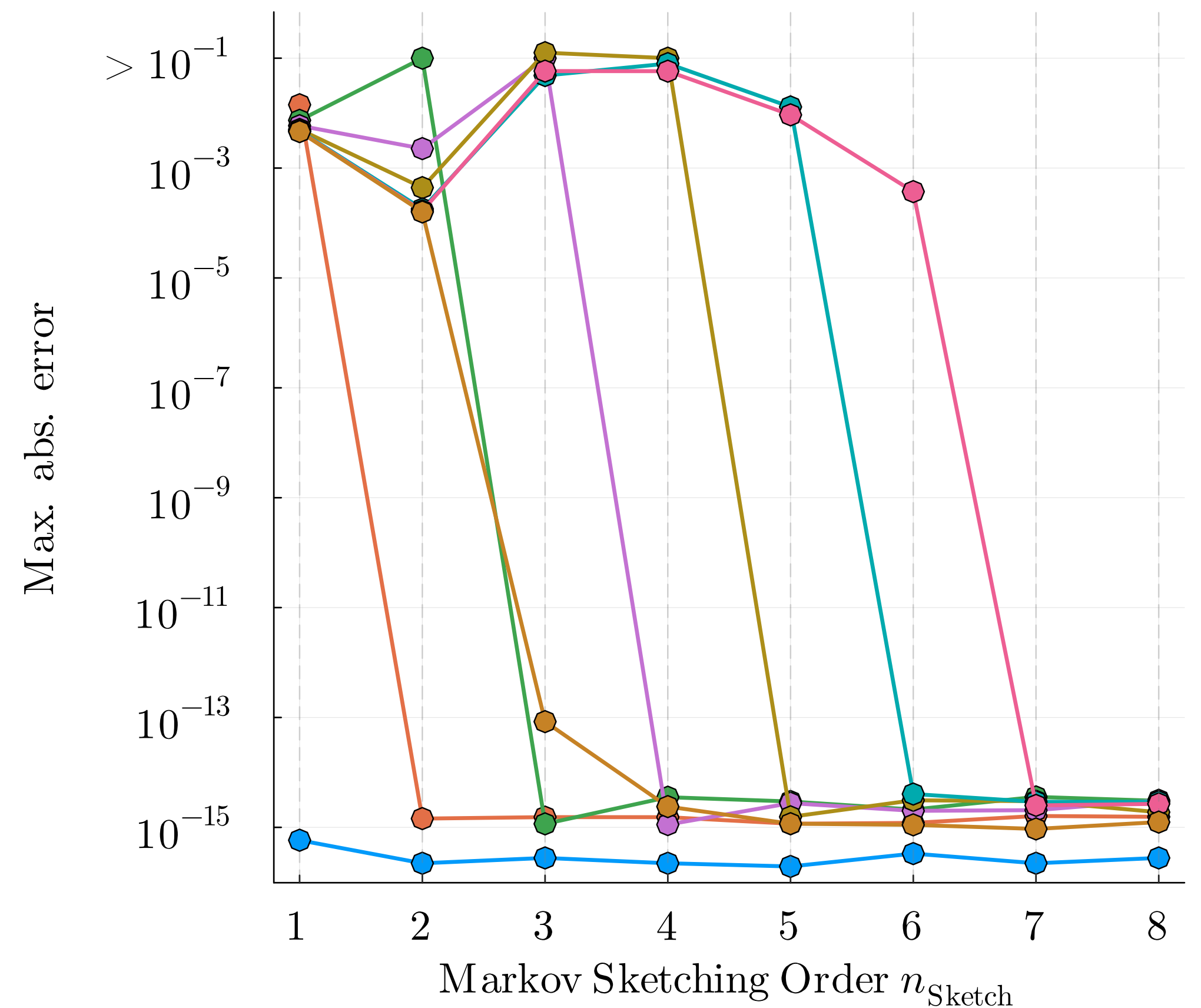
(b) Max. Abs. Error vs. Markov Sketching Order n_{\text{Sketch}}
