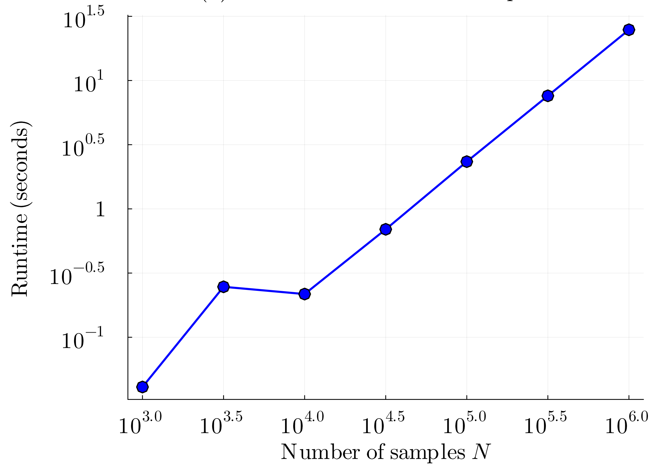
(b) Runtime vs. Number of samples N
