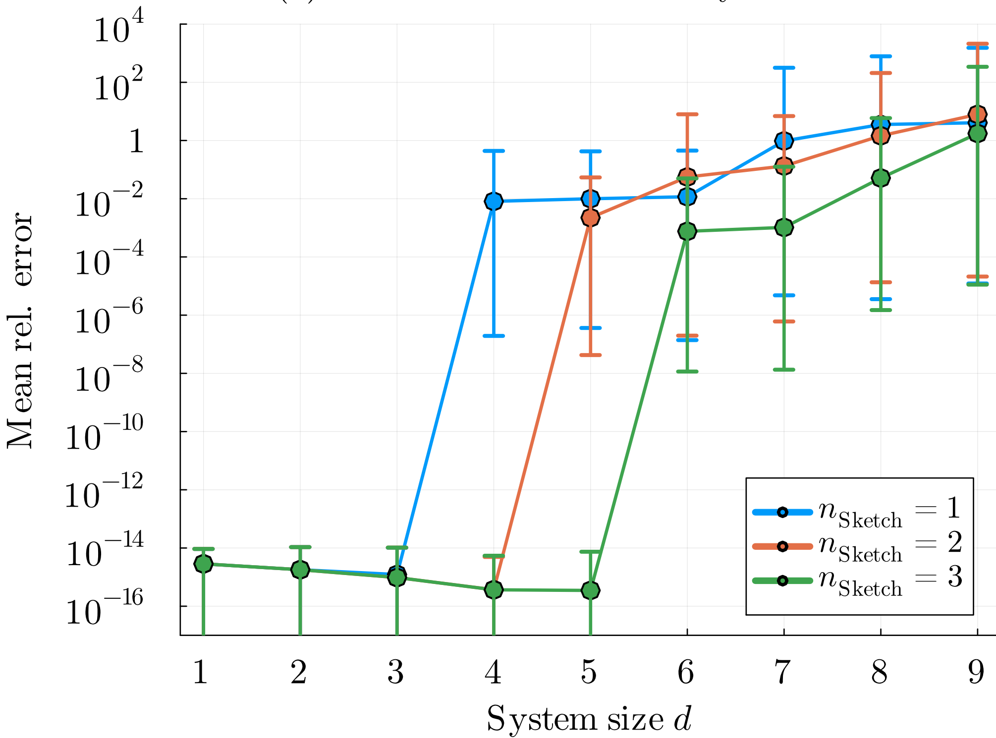
(a) Mean relative error vs. System size d
