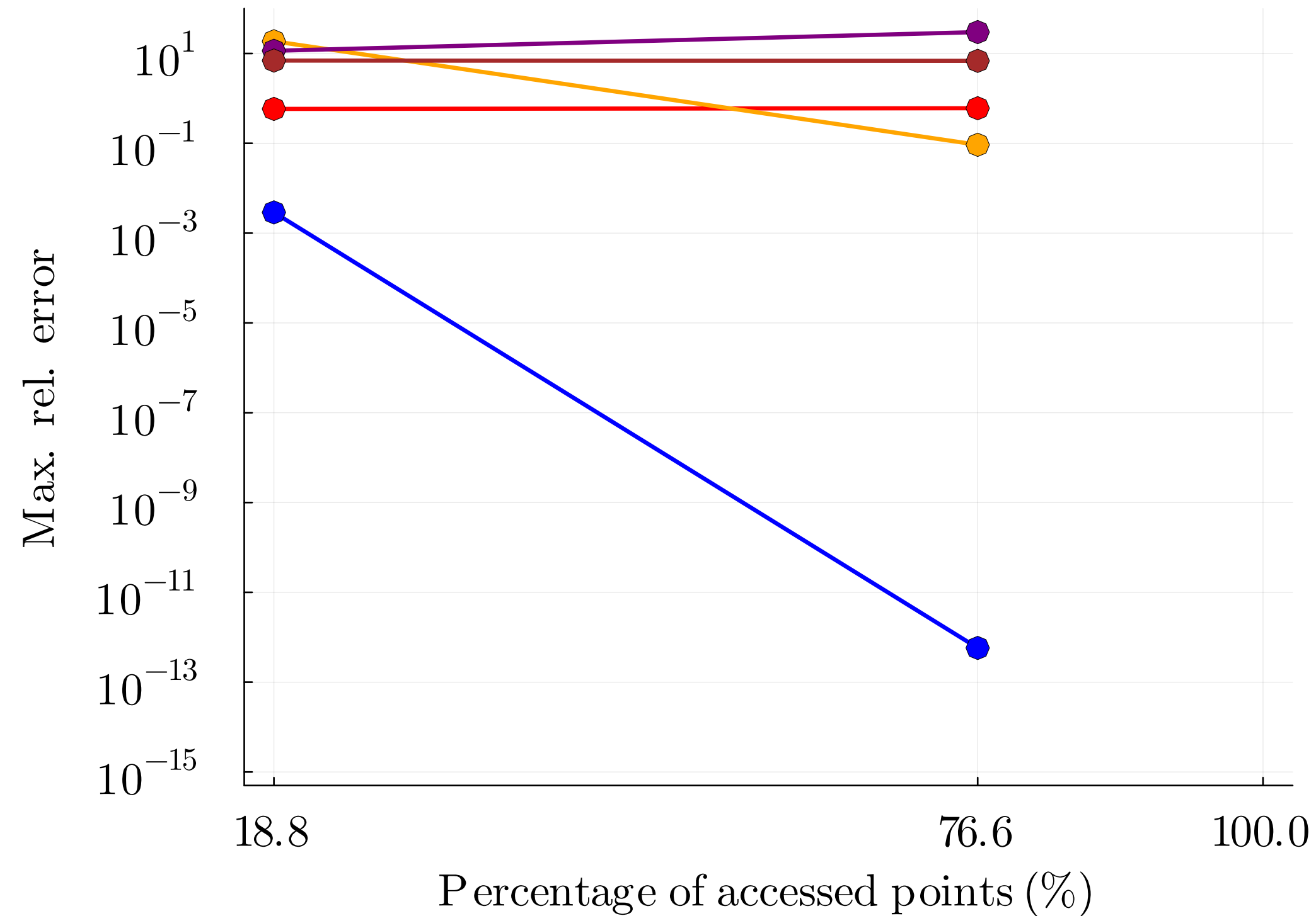
Unseen points : Max. rel. error vs. frac. accessed
