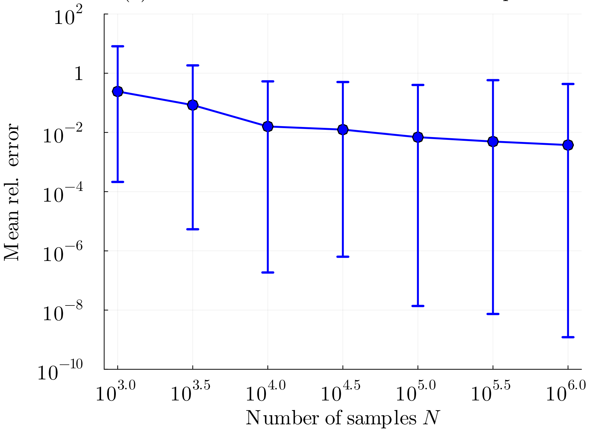
(a) Mean relative error vs. Number of samples N
