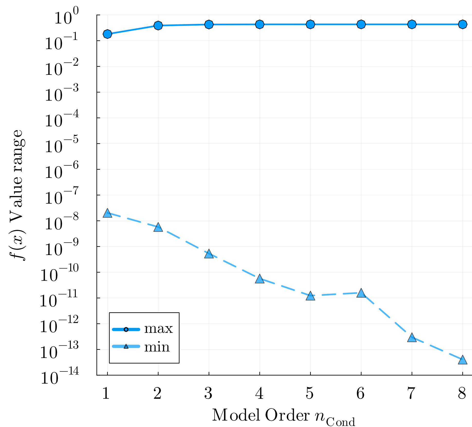
(c) Function value range vs. Model Order n_{\text{Cond.}} = n_{\text{Sketch}}
