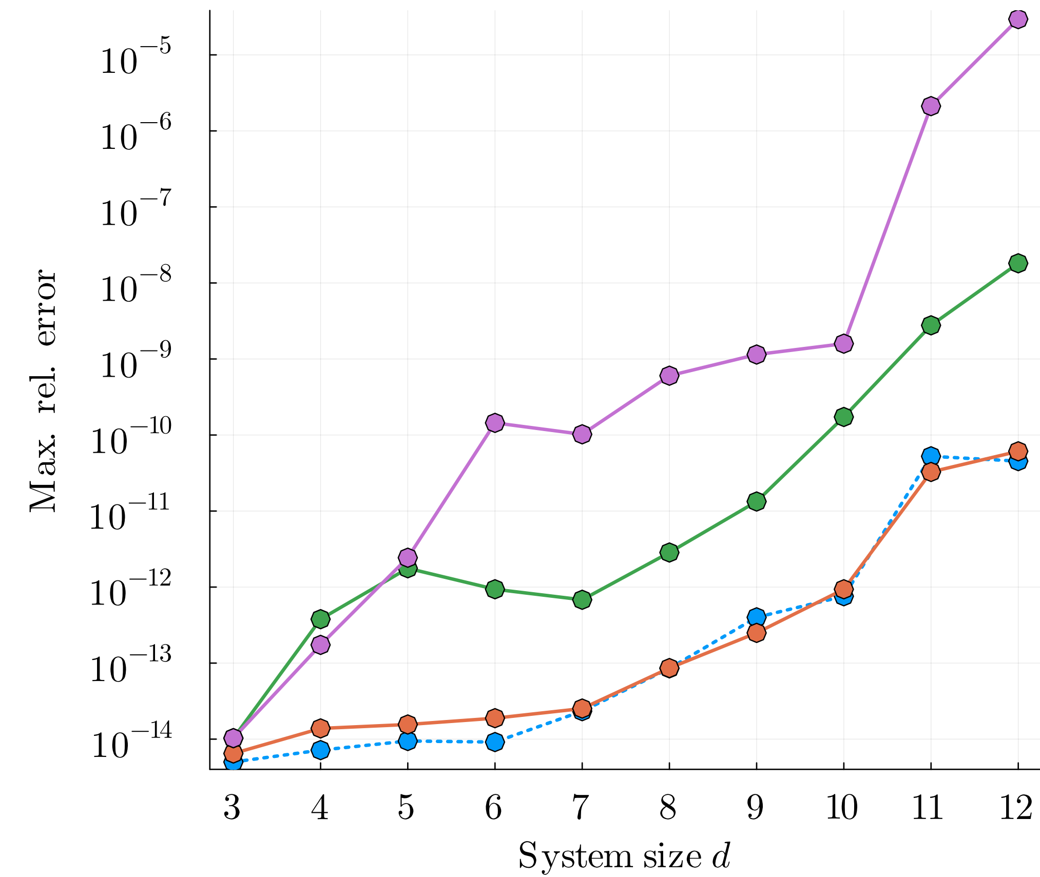
(a) Max. Rel. Error vs. System size d
