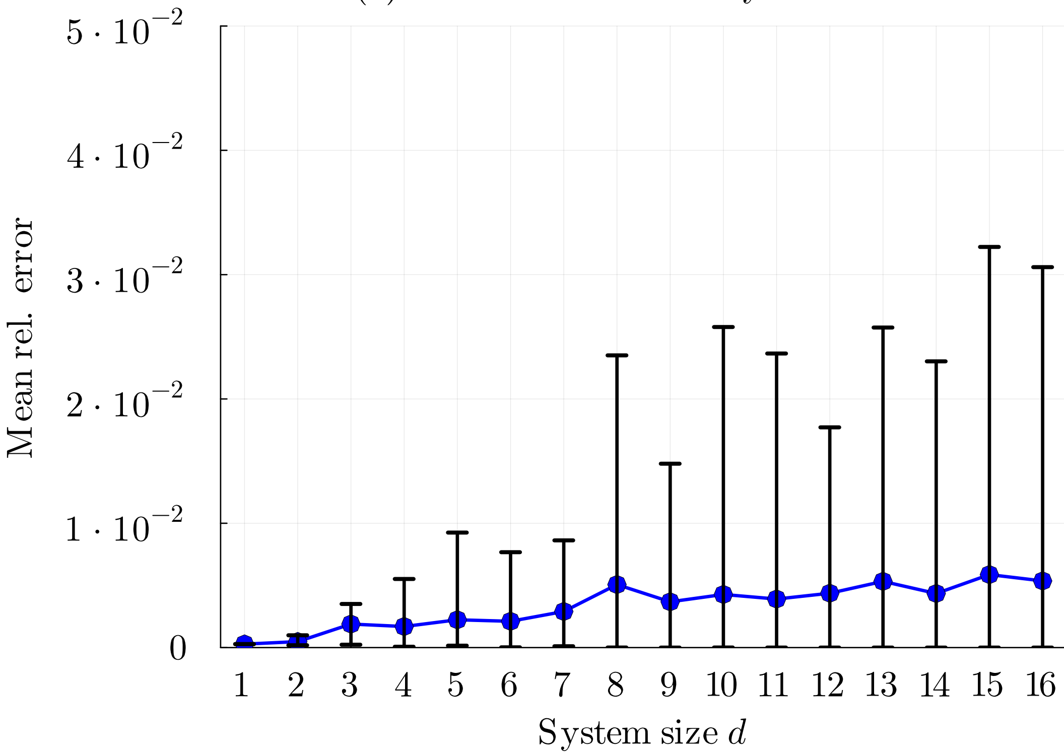
(a) Mean rel. error vs. System size d
