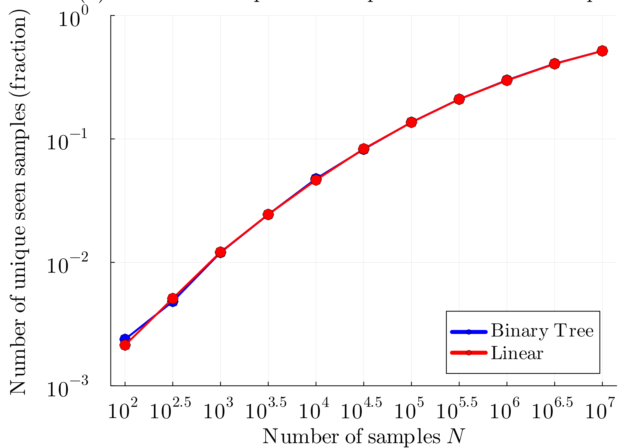
(b) Number of unique seen samples vs. Number of samples N
