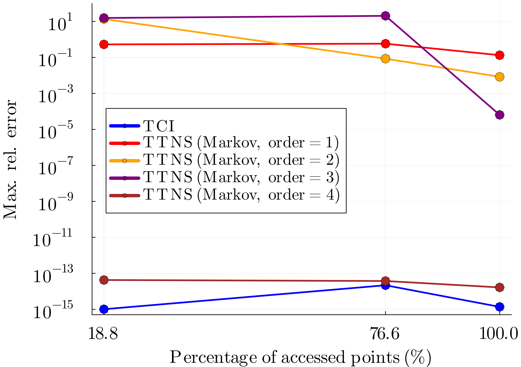
Seen points : Max. rel. error vs. frac. accessed points
