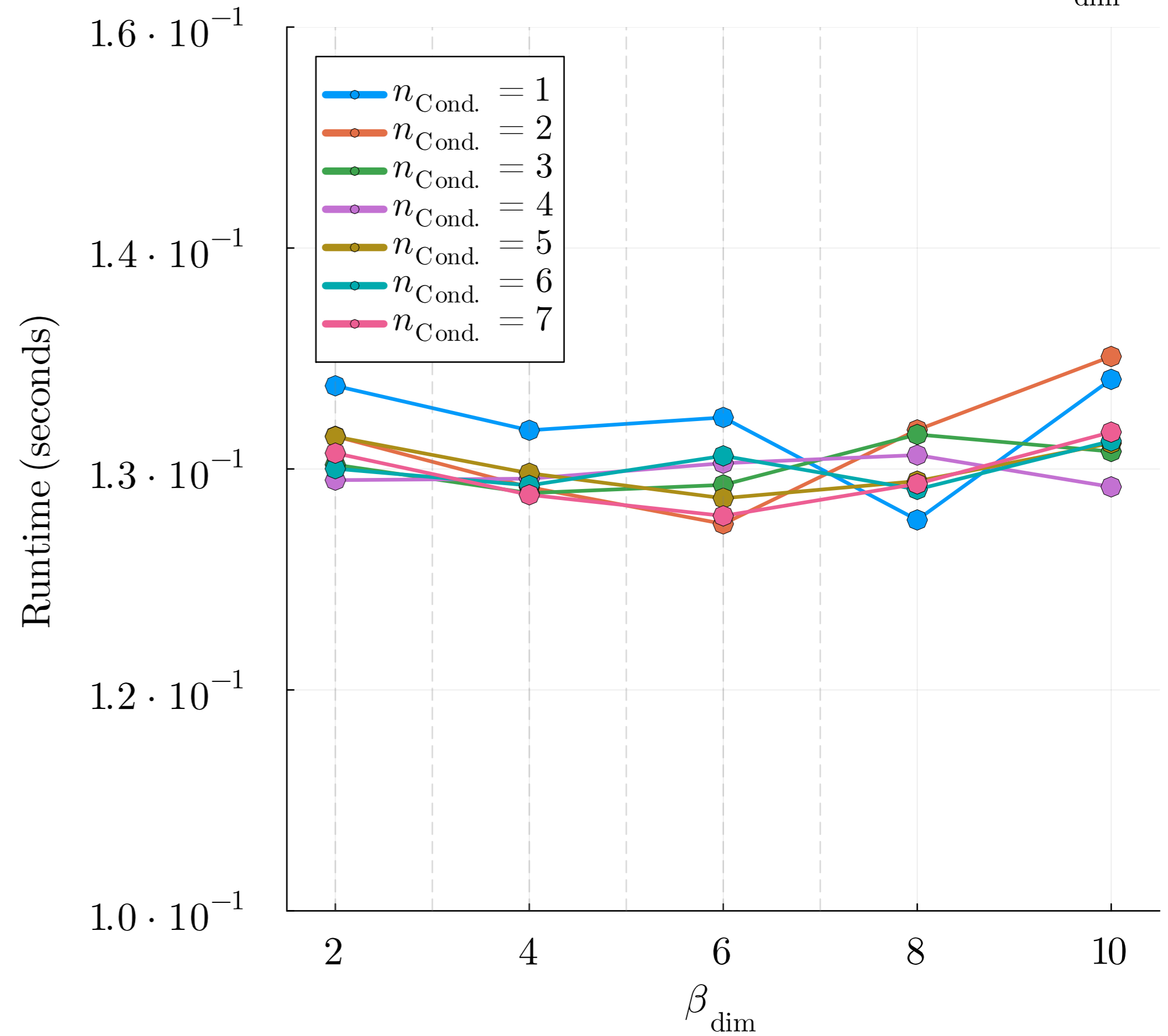
(b) Perturbative Sketching : Runtime vs. \beta_{\text{dim}}
