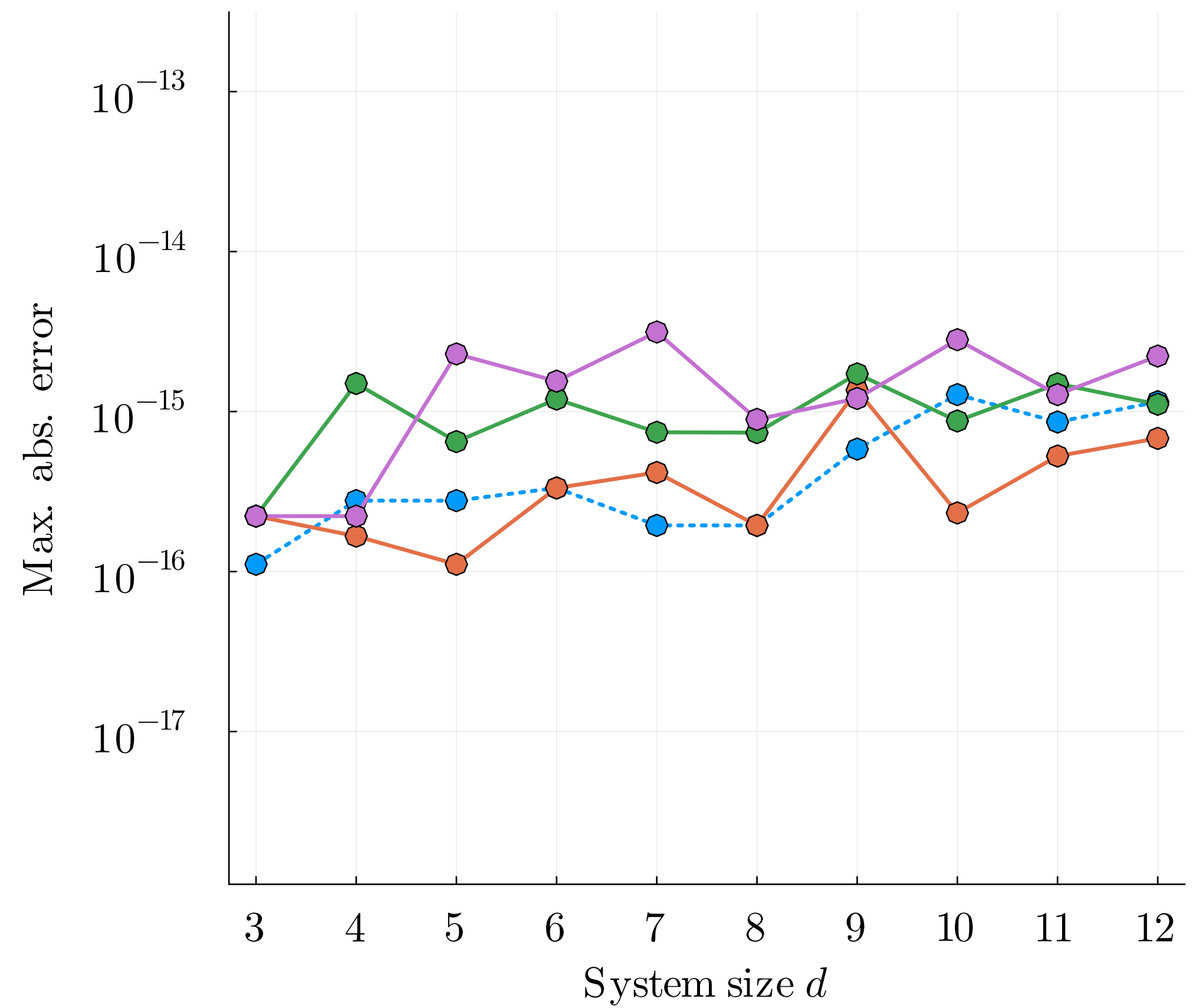
(b) Max. Abs. Error vs. System size d
