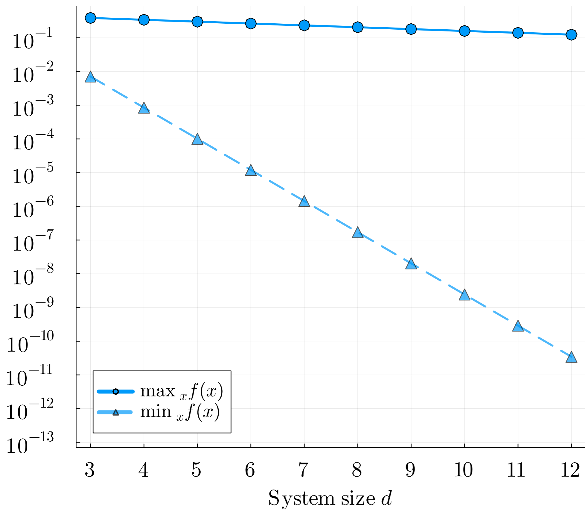
(c) f(x) Value range
