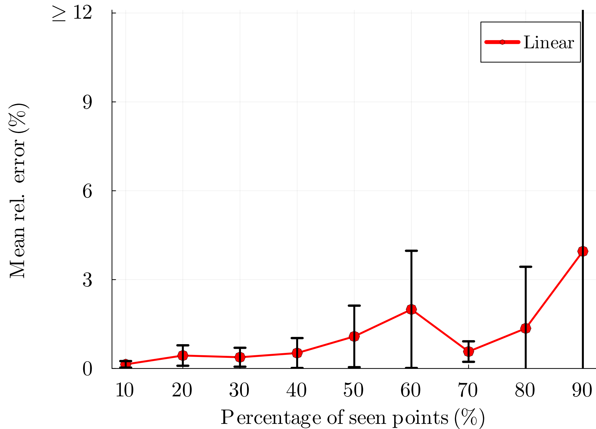
(b) Linear chain (15 vertices)
