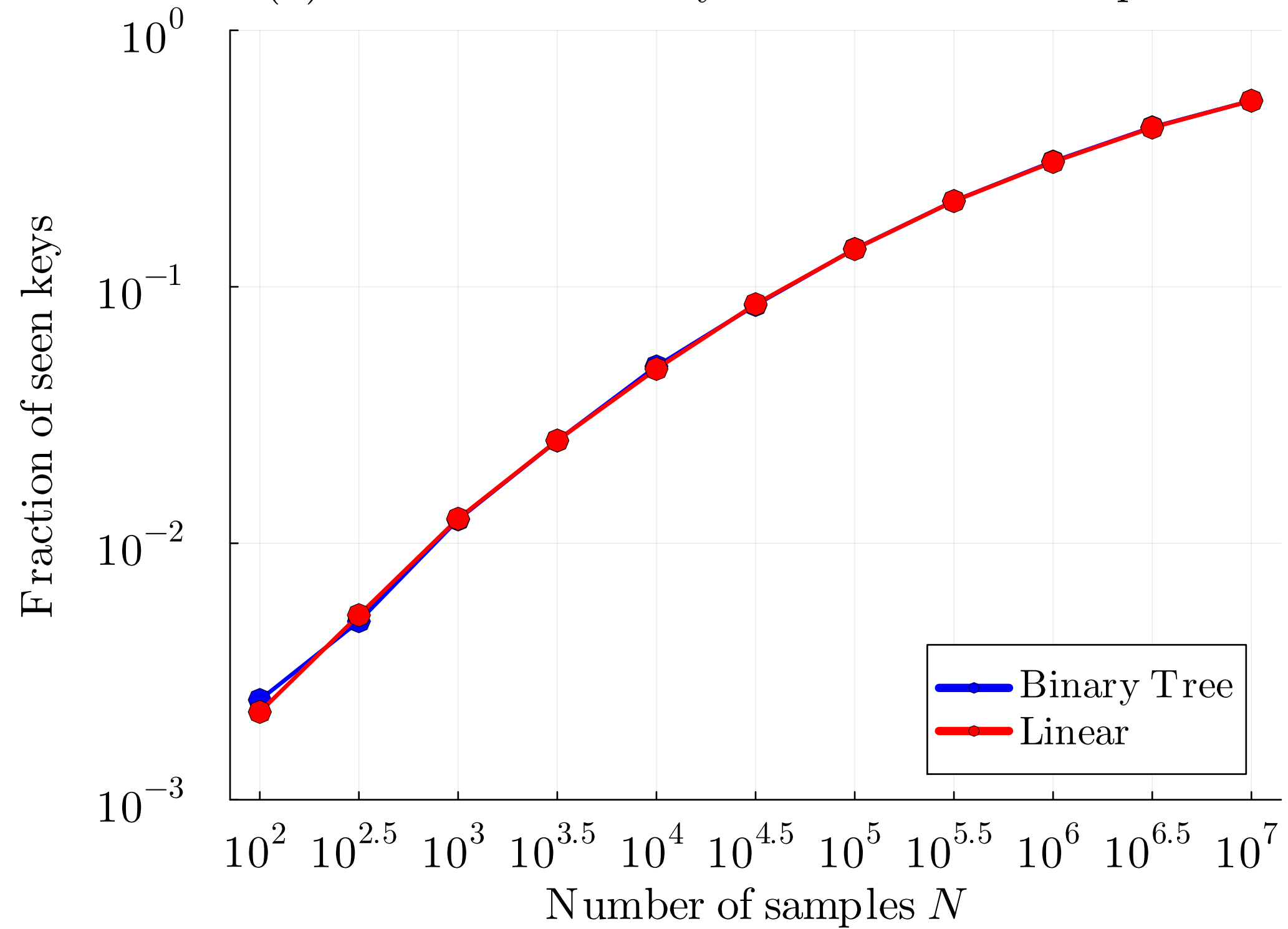
(b) Fraction of seen keys vs. Number of samples N
