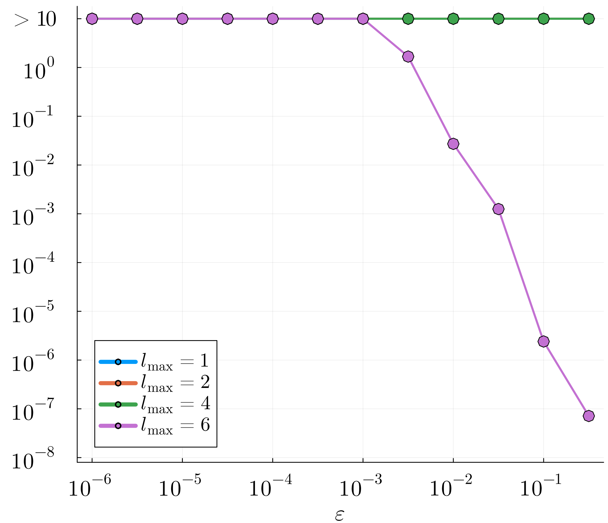
(b) Max. Rel. Error, n_{\text{Cond}} = 2
