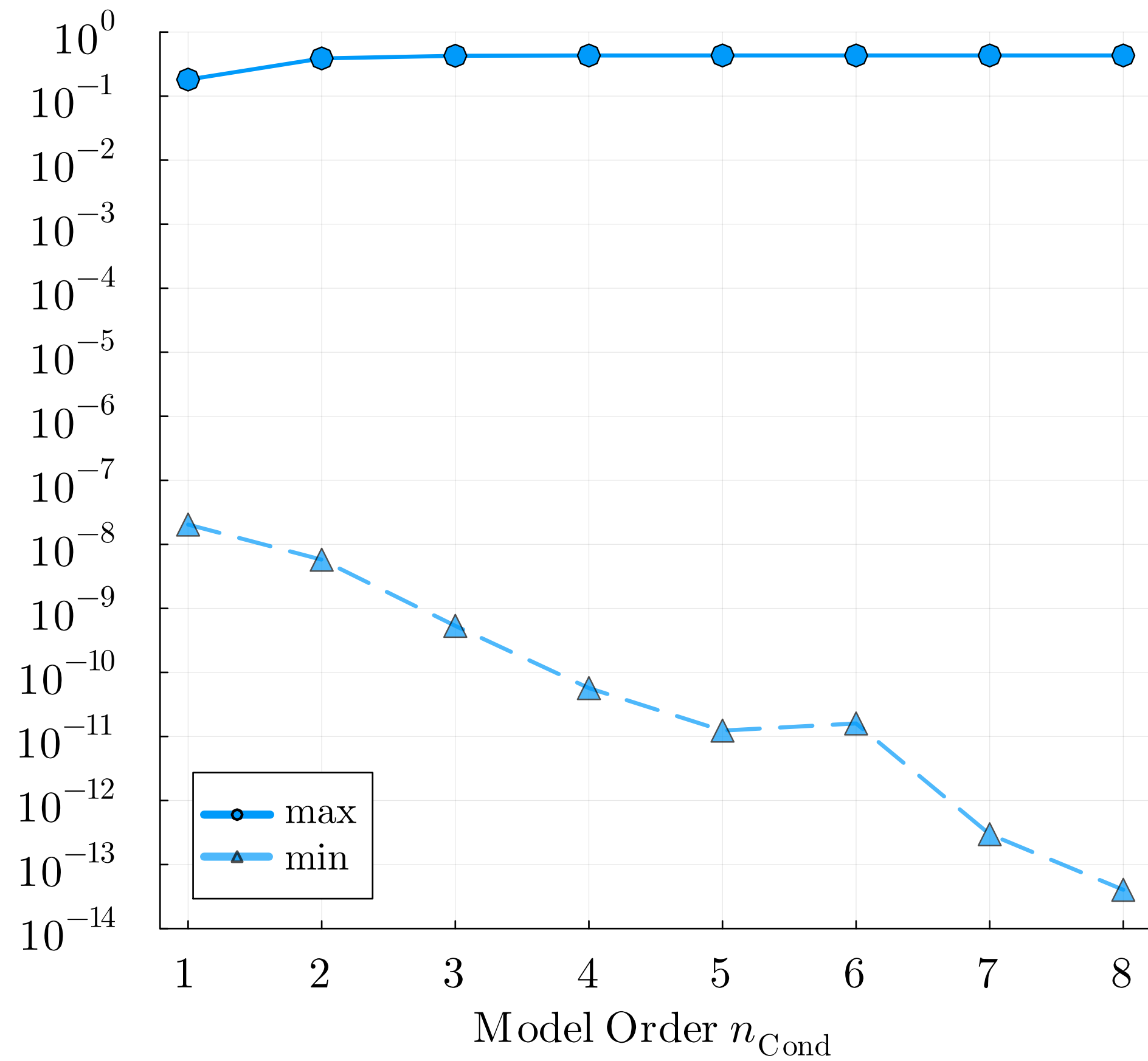
(c) f(x) Value range
