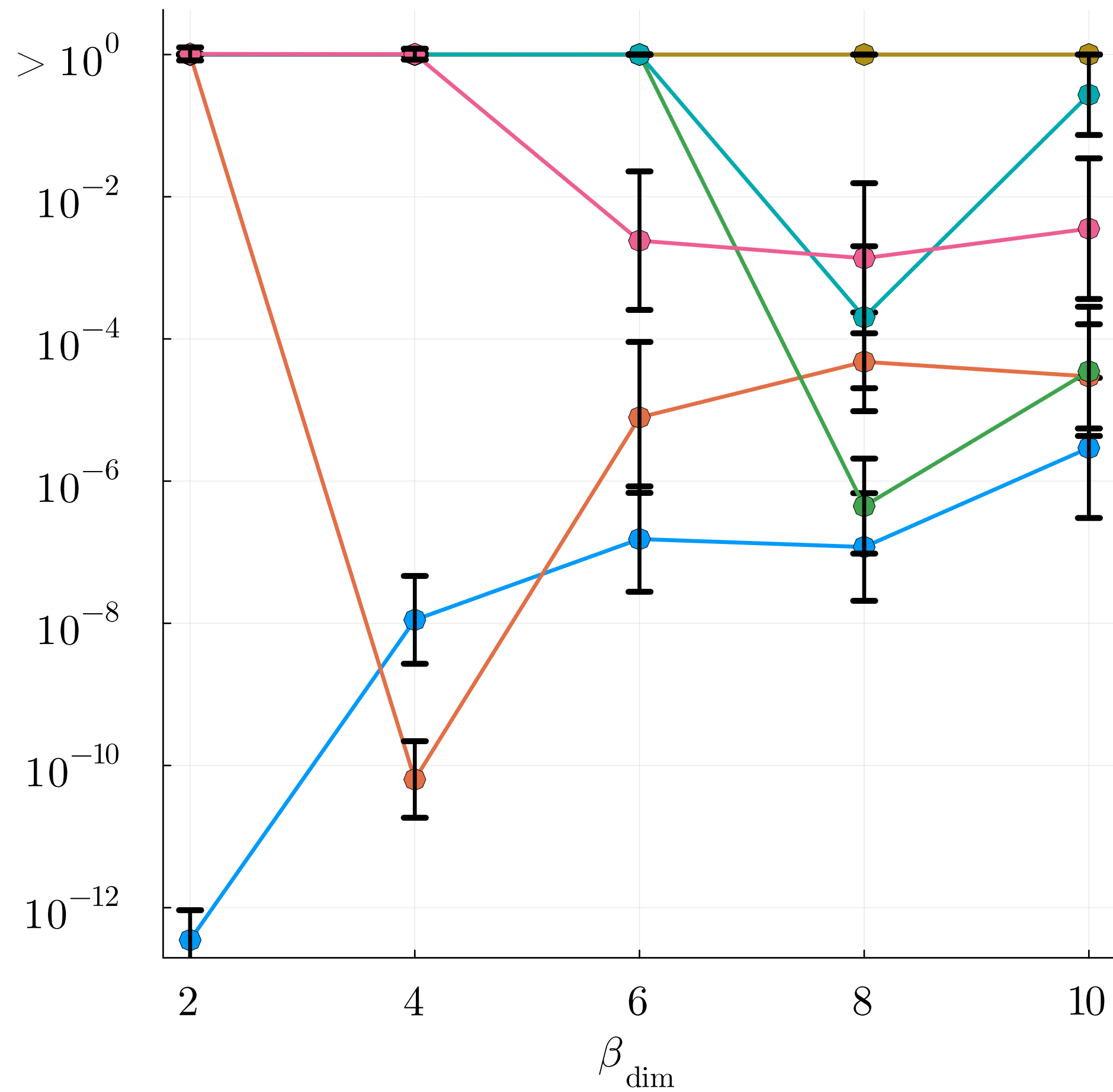
(a) Rel. Error \langle |(f(x) - f_{\text{ttns}}(x))| / f(x) \rangle
