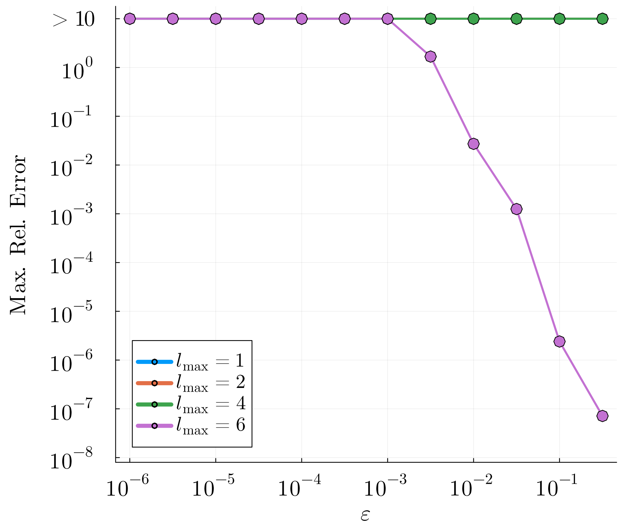
(b) Max. Rel. Error vs. \varepsilon , ( n_{\text{Cond.}} = 2 )
