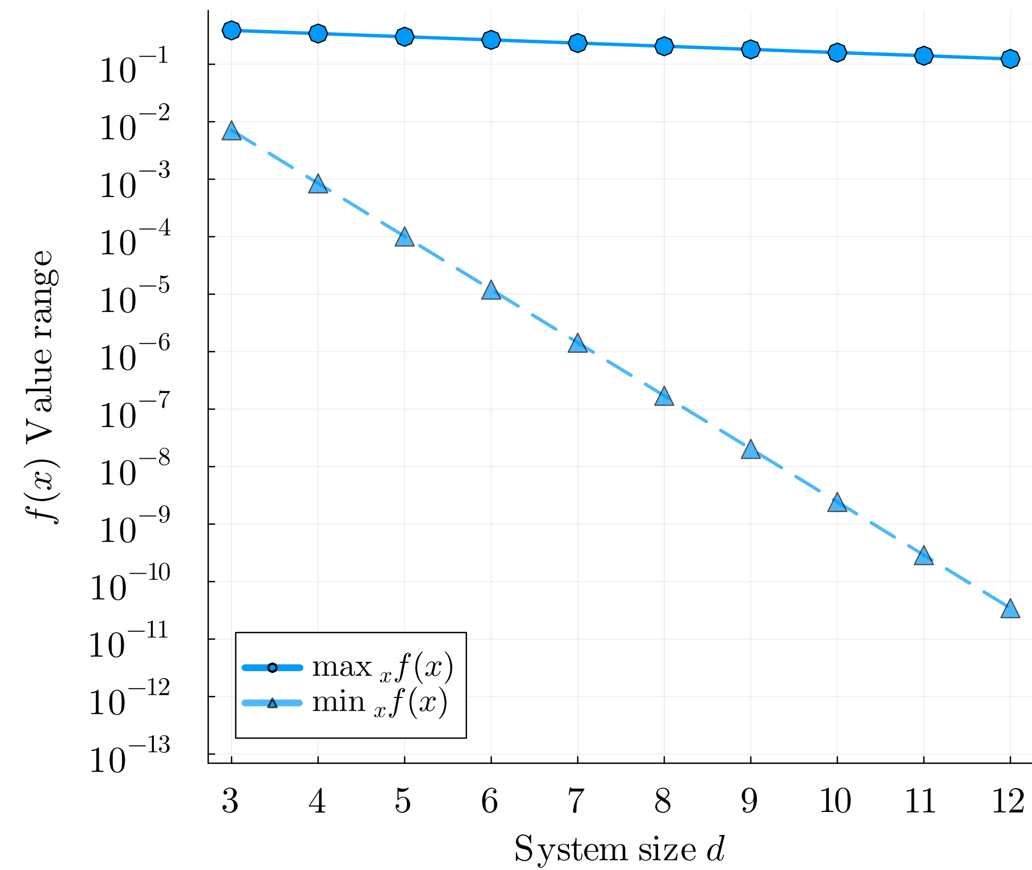
(c) Function value range vs. System size d
