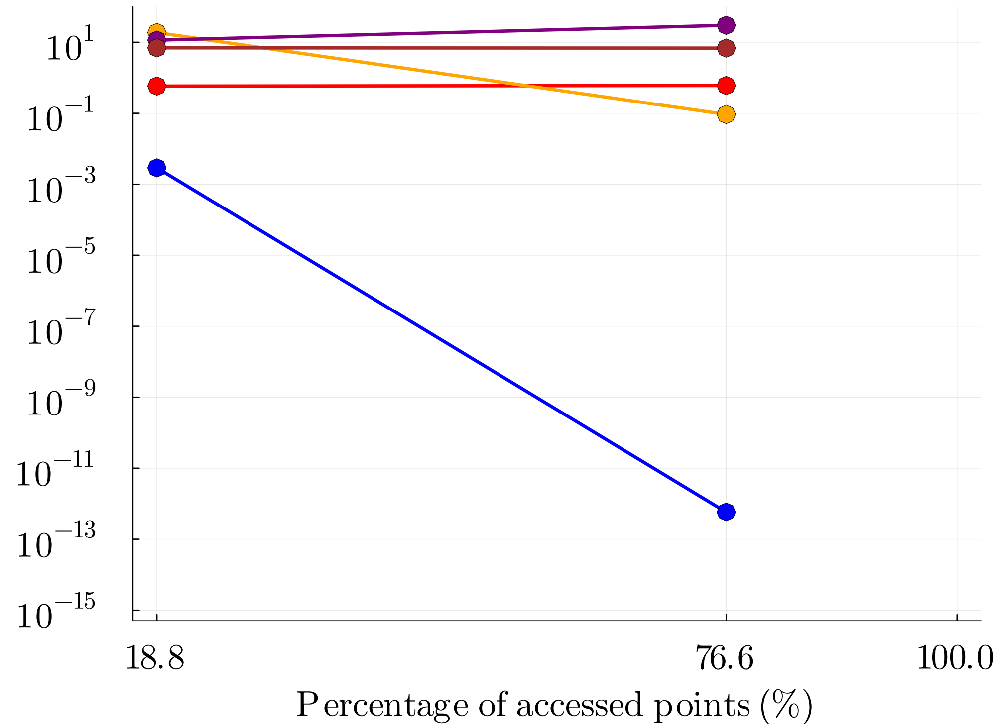
Unseen points : Max. rel. error vs. frac. accessed
