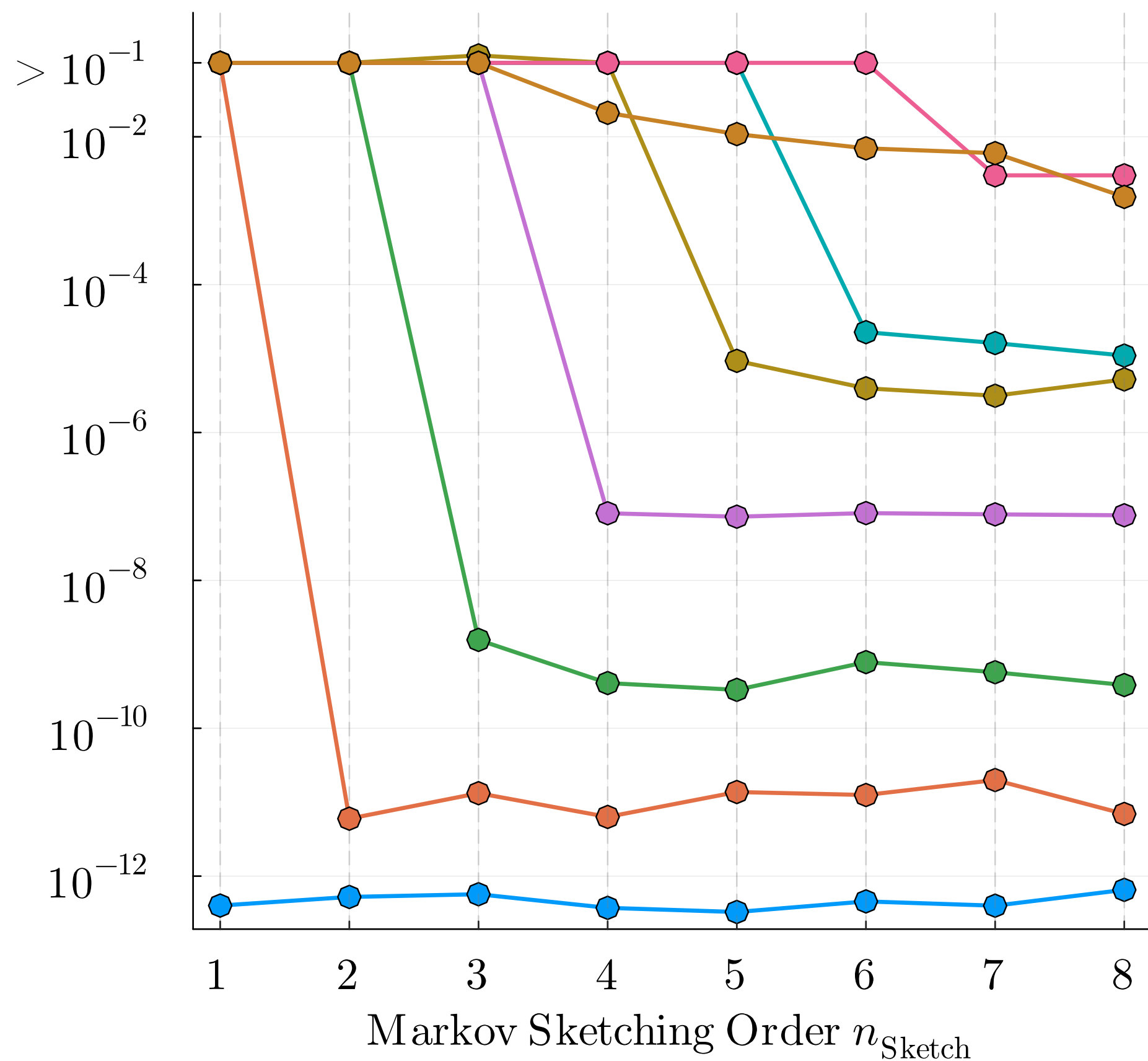
(a) Max. Rel. Error vs. Markov Sketching Order n_{\text{Sketch}}
