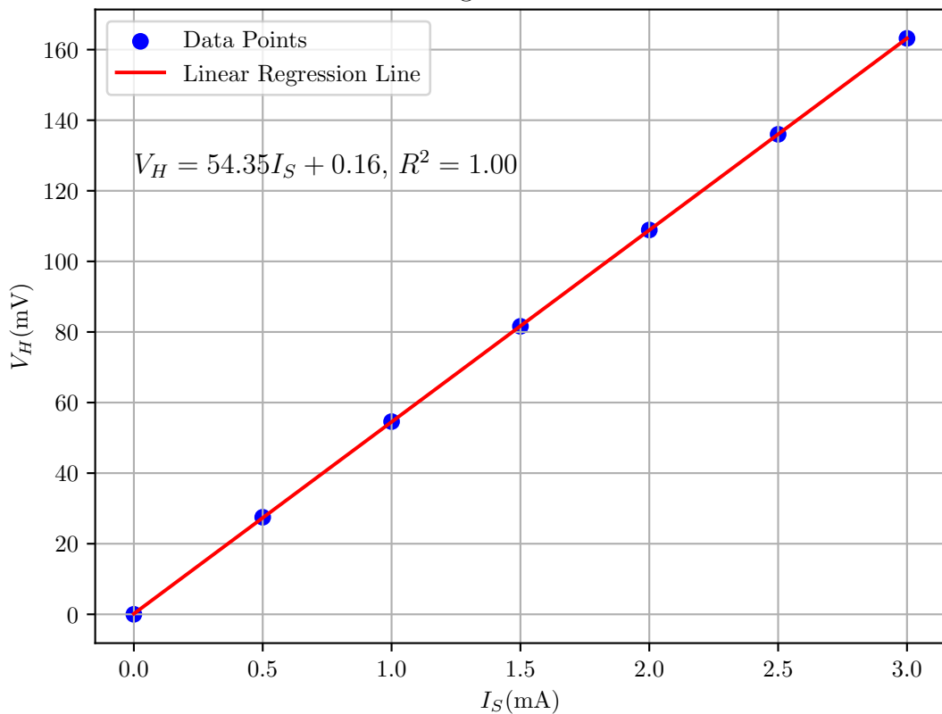
Linear Regression of V_H vs I_S
