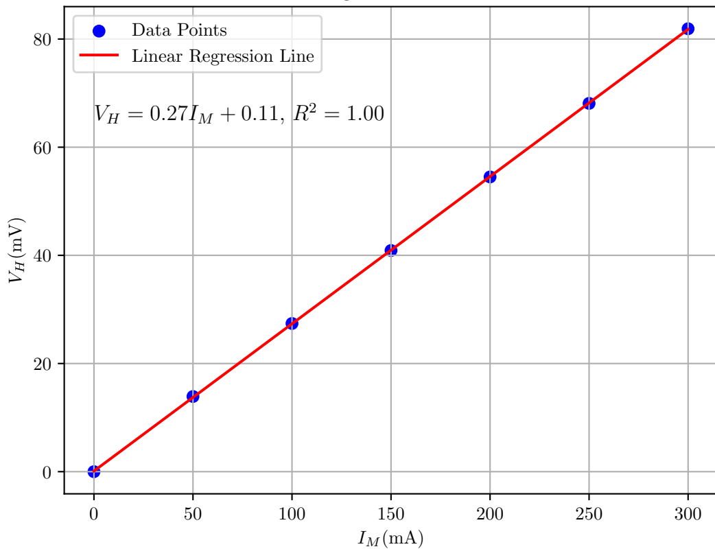
Linear Regression of V_H vs I_M
