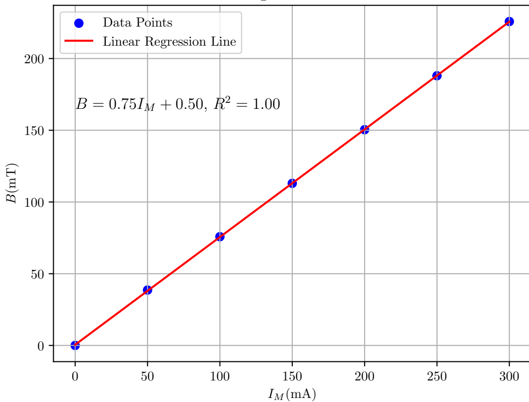
Linear Regression of B vs I_M
