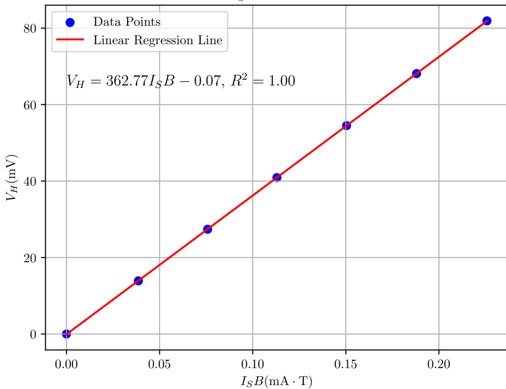
Linear Regression of V_H vs I_S B
