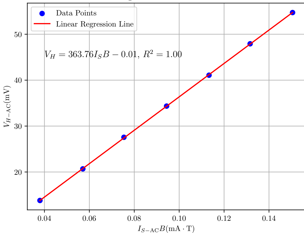
Linear Regression of V_{H-AC} vs I_{S-AC}B
