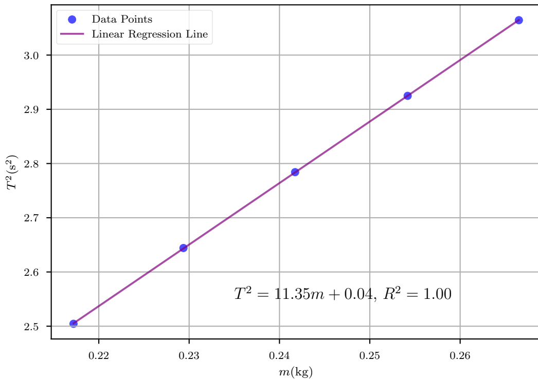
Linear Regression (Least Squares Method) of T^2 vs m
