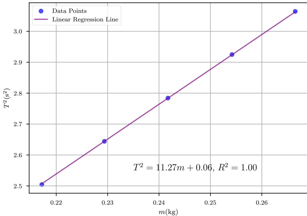
Linear Regression (Ridge with \alpha = 1e-5 ) of T^2 vs m
