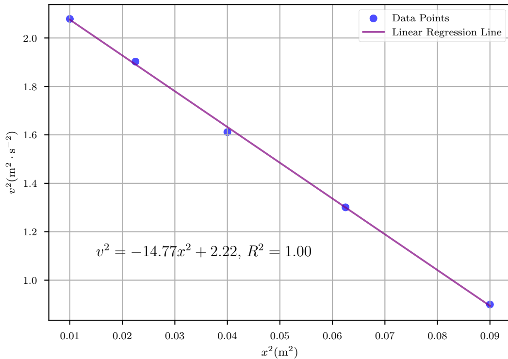
Linear Regression (Least Squares Method) of v^2 vs x^2
