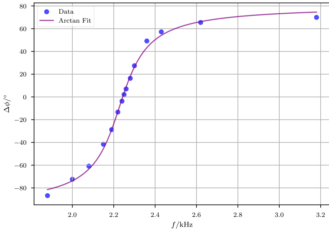
\Delta\phi \sim f Curve
