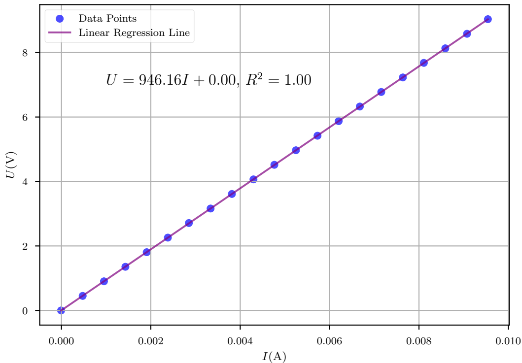
Linear Regression (Least Squares Method) of U vs I
