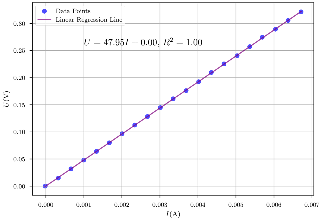
Linear Regression (Least Squares Method) of U vs I
