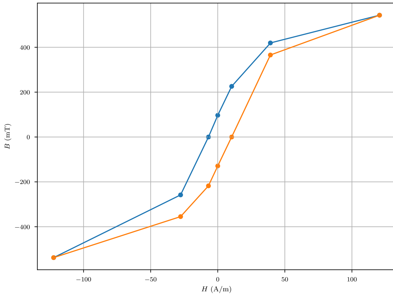
Saturation Dynamic Hysteresis Loop of Ferrite
