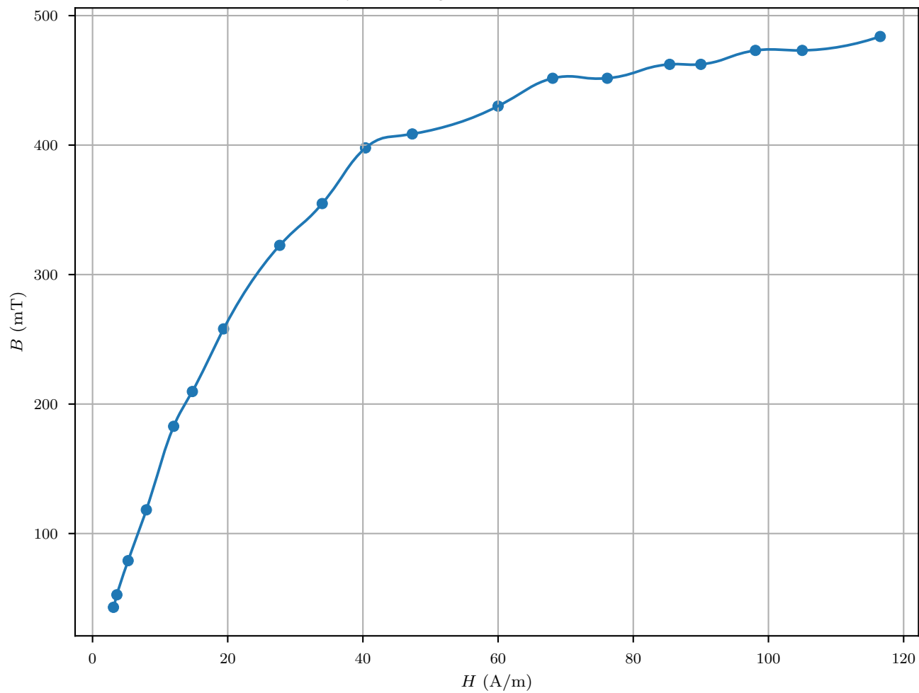
Dynamic Magnetization Curve of Ferrite
