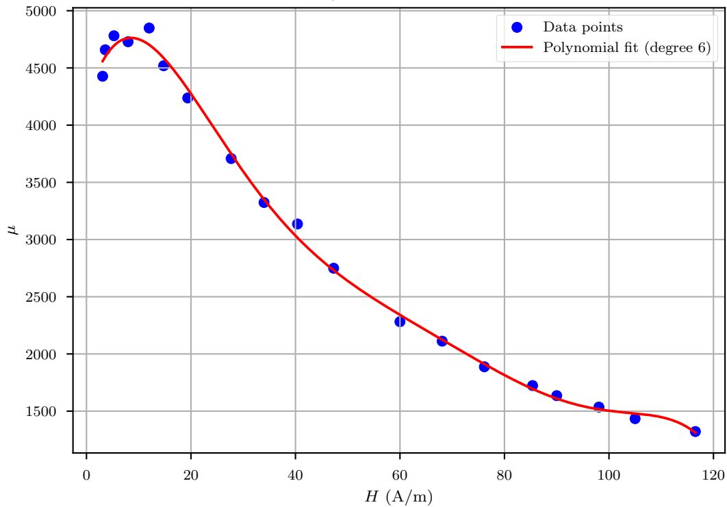
\mu vs H of Ferrite
