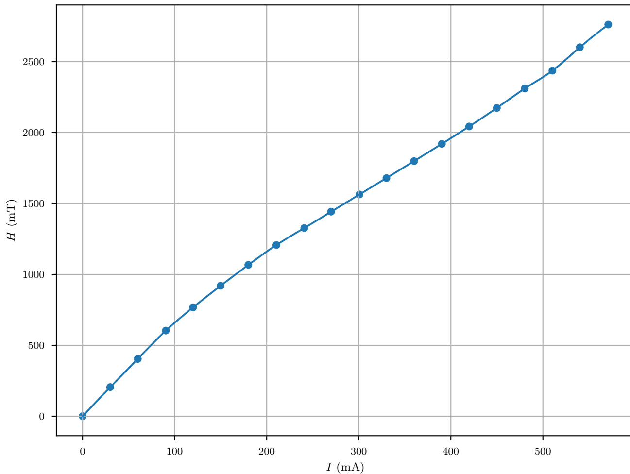
The Starting Magnetization Curve of a Mold Steel Sample
