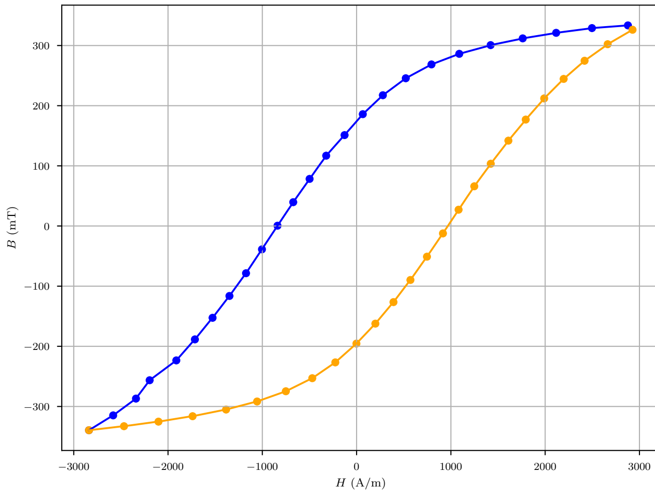
The Hysteresis Loop of a Mold Steel Sample
