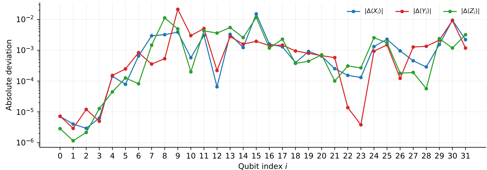
N=32 warm-start sewing vs target: local observable deviations
