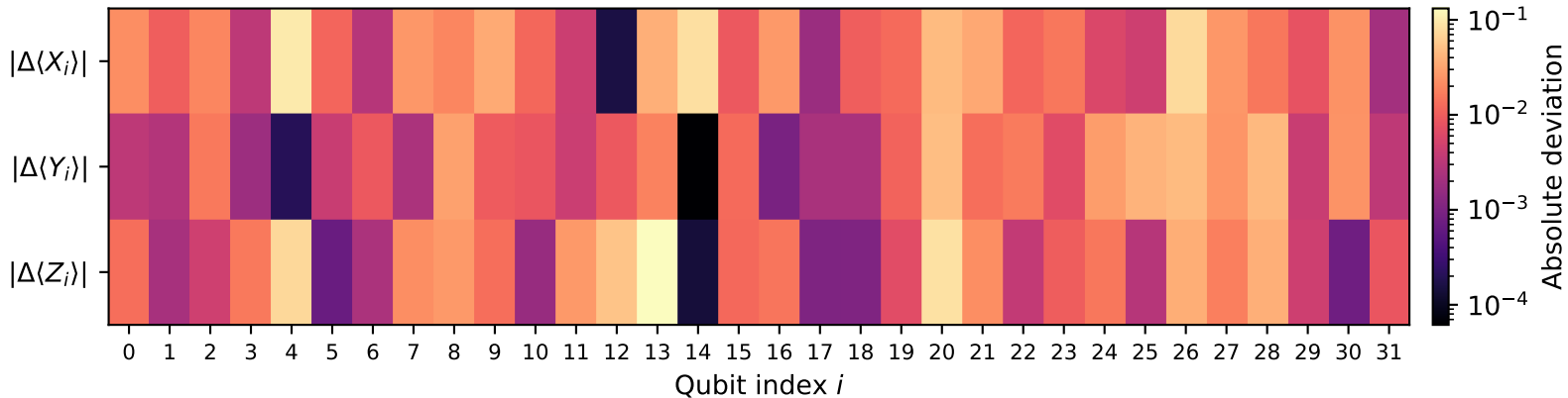
N=32 mixed-channel sewing vs target: deviation heatmap
