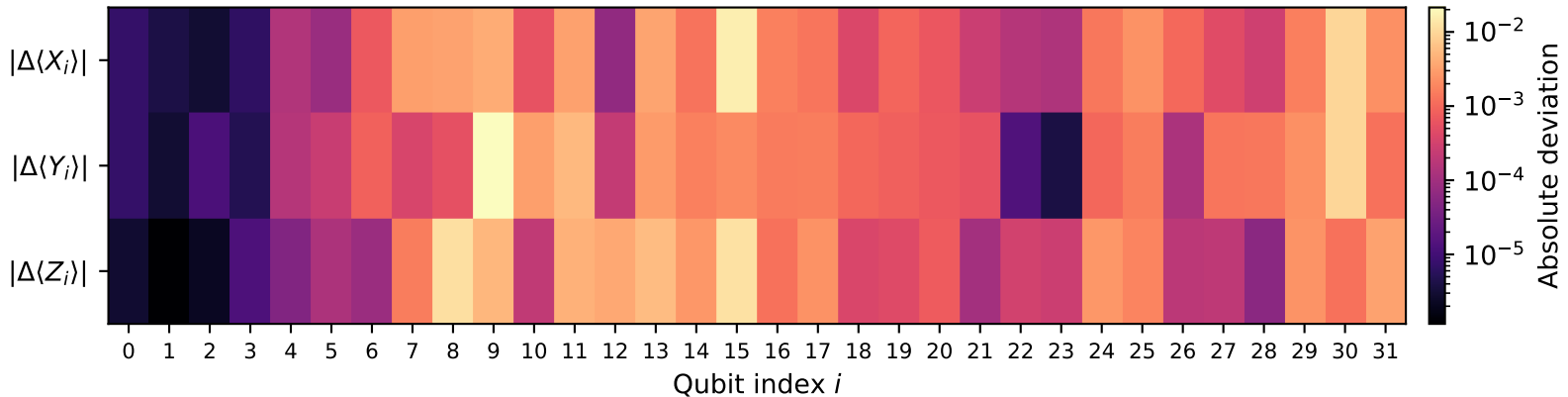
N=32 warm-start sewing vs target: deviation heatmap
