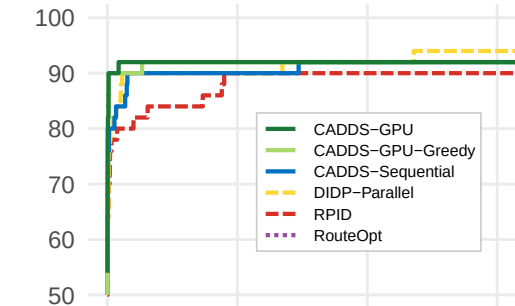
Solnon (Feasible)
