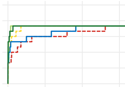
Solomon-Potvin-Bengio
