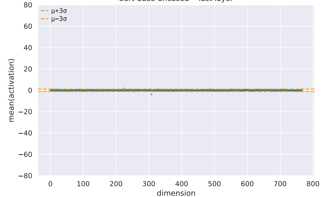
bert-base-uncased • last layer
