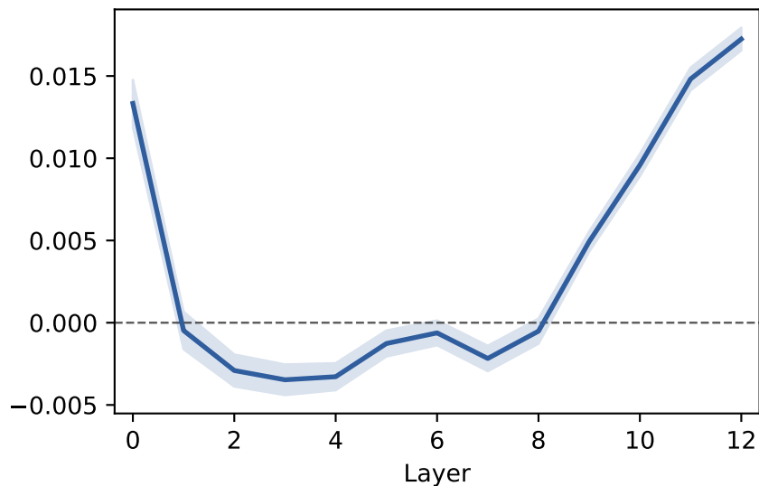
IsoScore
