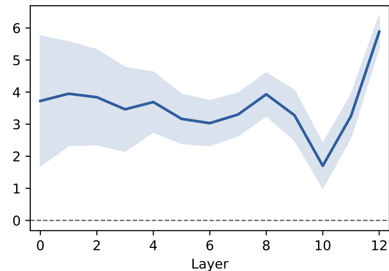
Nonlinear ID
