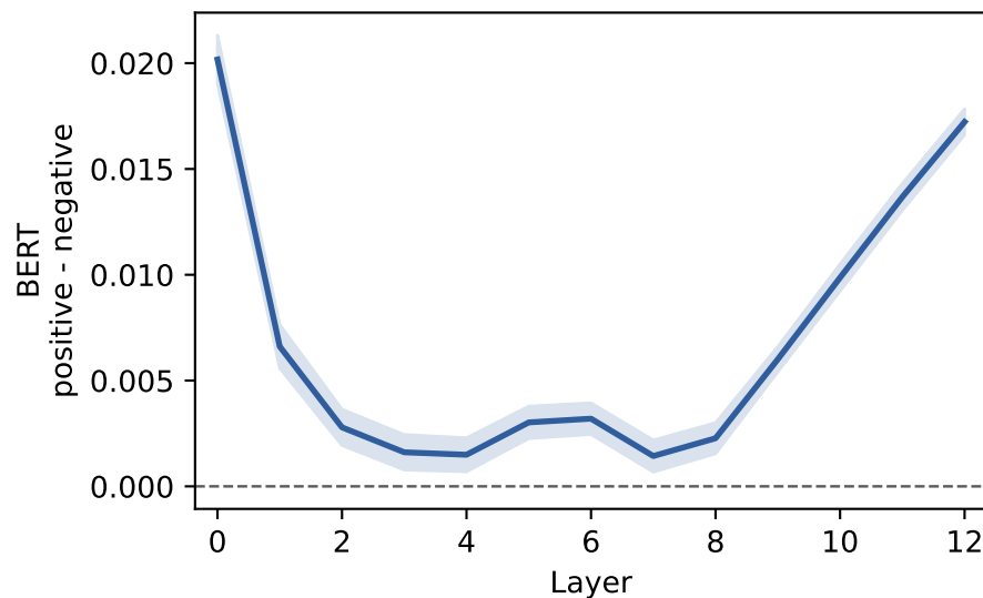
IsoScore
